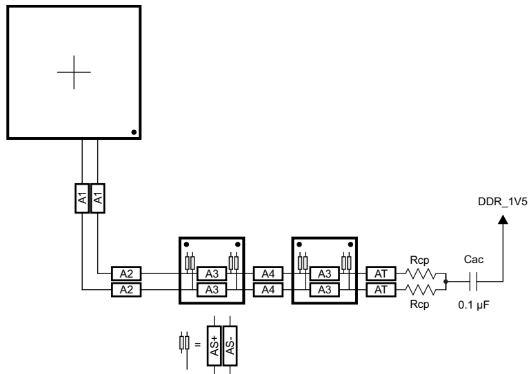
7-66. CK Routing for Four Mirrored DDR3 Devices
