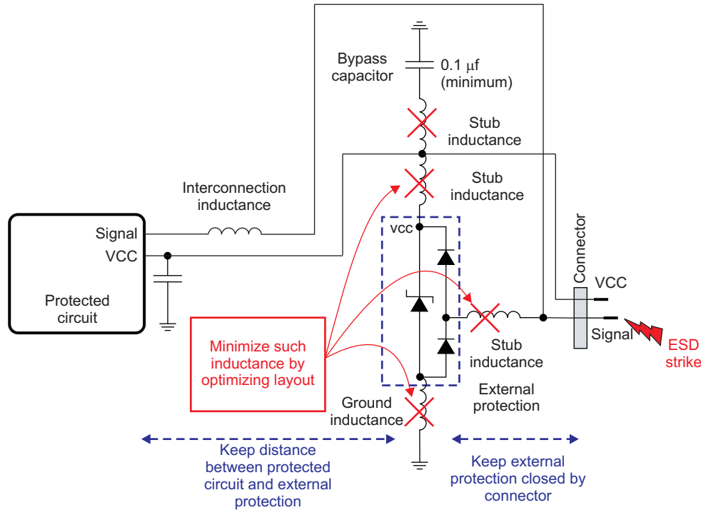
☒ 7-16. Placement Recommendation for an ESD External Protection
