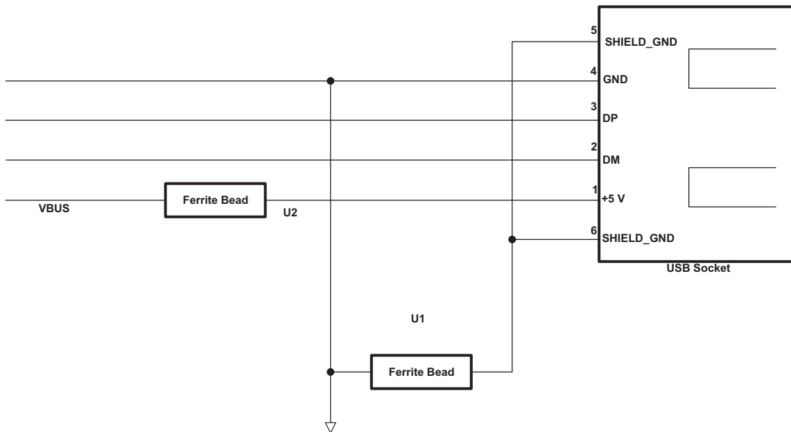
7-32. USB Connector
