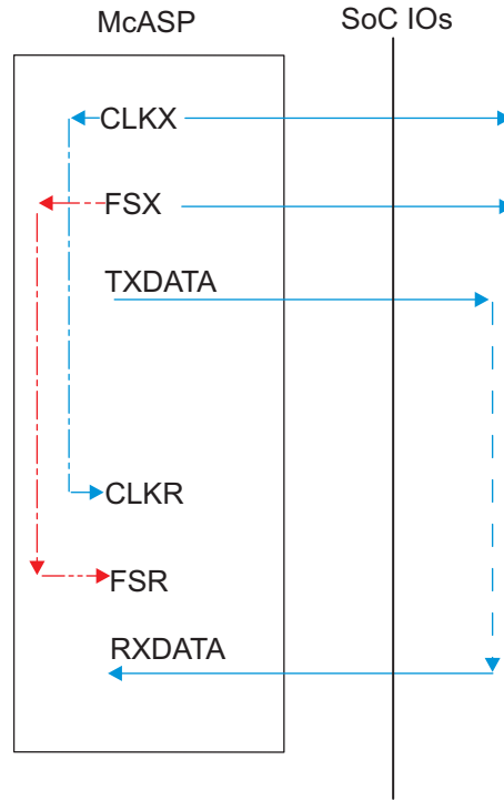
Figure 5-61. McASP1-8 CO-FO- – SYNC Mode
