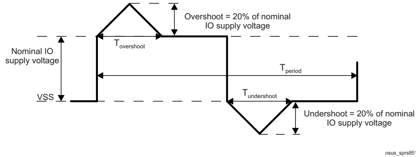
5-1. T_{overshoot} + T_{undershoot} < 20\% of T_{period}
