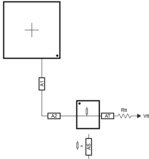
SPRS906_PCB_DDR3_21
