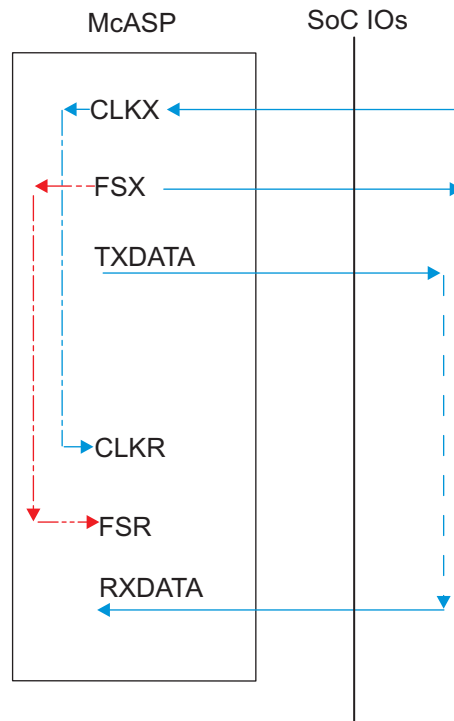
Figure 5-62. McASP1-8 CI-FO- – SYNC Mode
