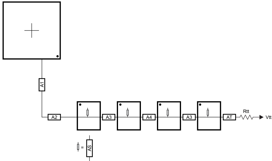
7-65. ADDR_CTRL Routing for Four Single-Side DDR3 Devices
