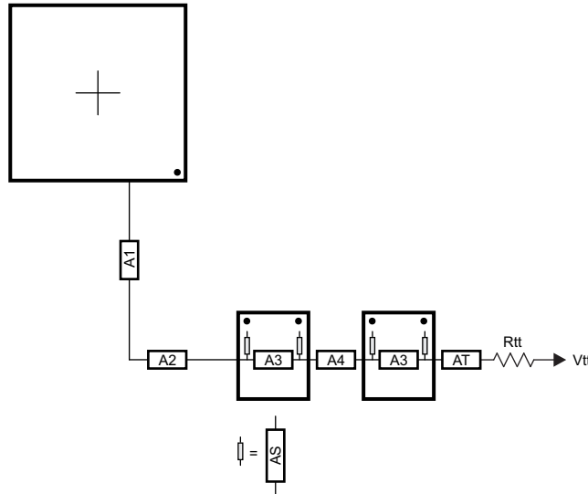
SPRS906_PCB_DDR3_11
