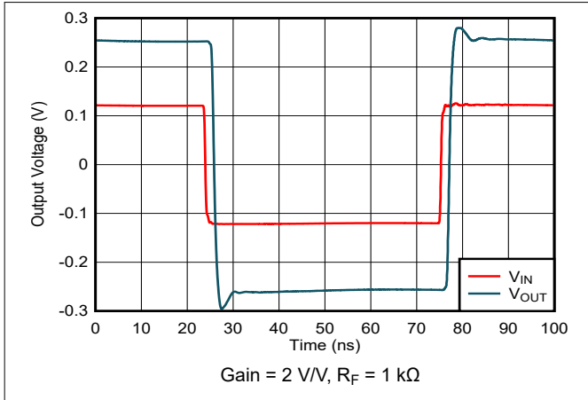
7-25. Noninverting Small-Signal Transient Response
