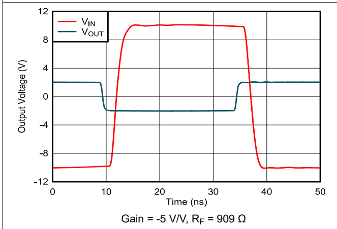
7-27. Inverting Large-Signal Transient Response
