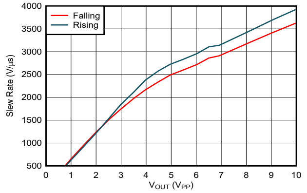
7-14. Slew Rate vs Output Voltage Step
