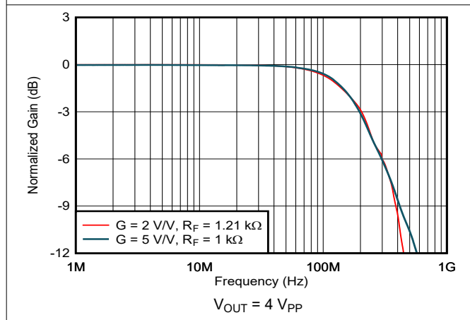
7-5. Noninverting Large-Signal Frequency Response
