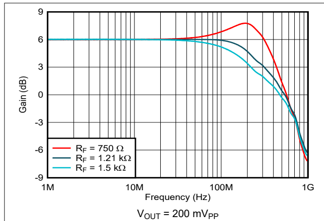
7-1. Noninverting Small-Signal Frequency Response
