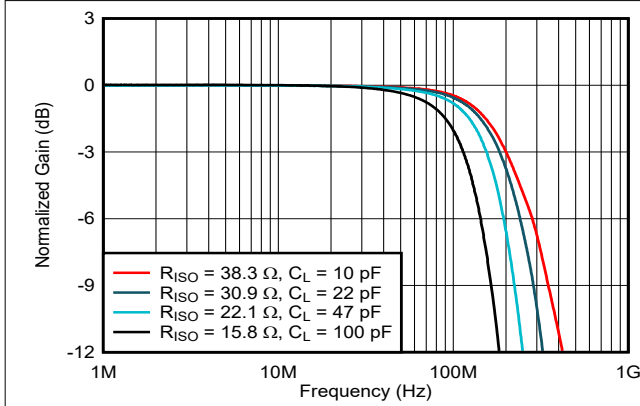
7-7. Capacitive Load Frequency Response
