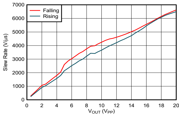
7-13. Slew Rate vs Output Voltage Step
