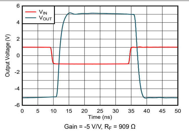
7-26. Inverting Large-Signal Transient Response
