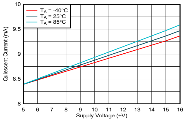
7-19. Quiescent Current vs Supply Voltage
