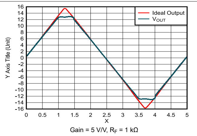
7-28. Output Overdrive Recovery Time
