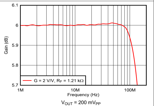
7-4. 0.1-dB Gain Flatness Frequency Response
