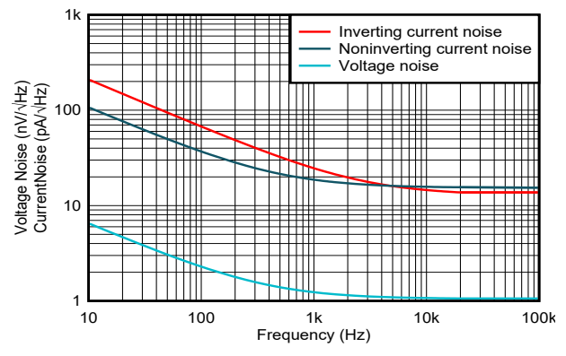
7-16. Noise vs Frequency
