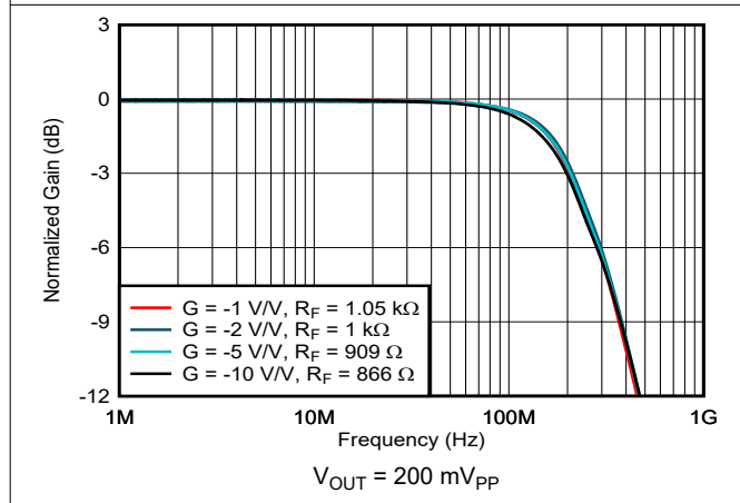
7-3. Inverting Small-Signal Frequency Response
