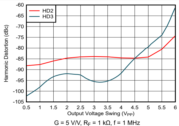
7-37. Harmonic Distortion vs Output Voltage Swing
