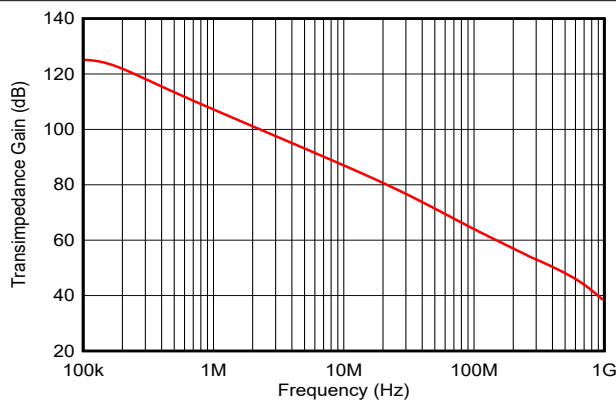
7-23. Transimpedance vs Frequency
