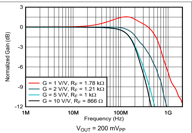
7-2. Noninverting Small-Signal Frequency Response
