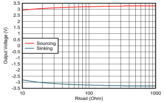
7-39. Output Voltage vs Load Resistance
