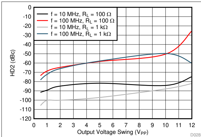
8-48. HD2 vs Output Swing
