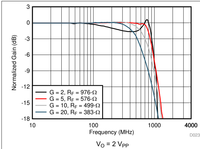
8-42. Noninverting Small-Signal Frequency Response
