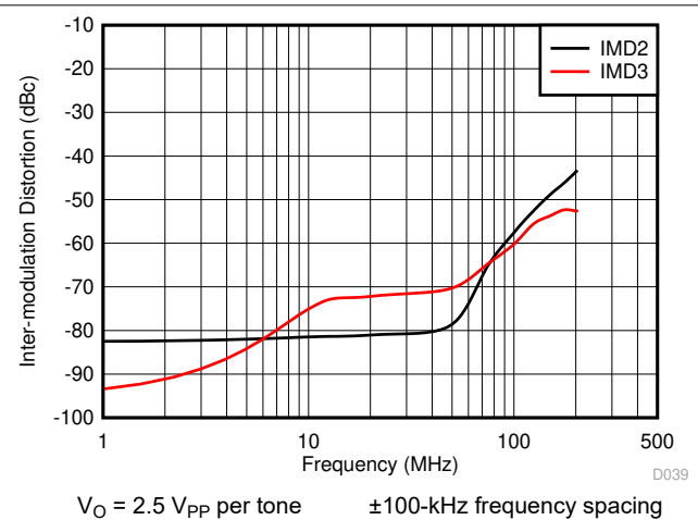
8-51. Intermodulation Distortion vs Frequency
