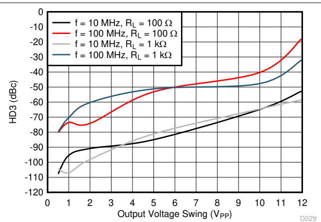
8-49. HD3 vs Output Swing
