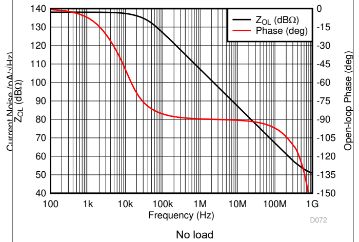
8-22. Open-Loop Transimpedance Gain and Phase vs Frequency
