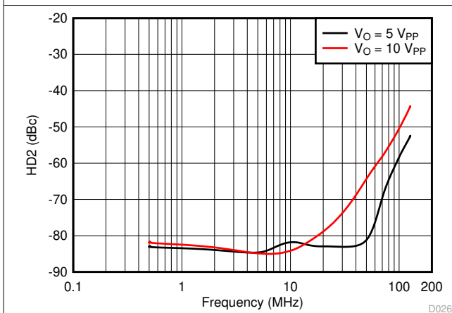
8-46. HD2 vs Frequency Across Output Swing
