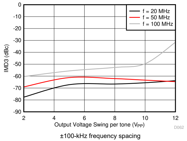
8-20. IMD3 vs Output Voltage Swing
