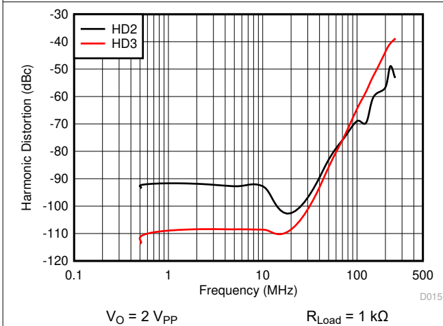
8-17. Harmonic Distortion vs Frequency
