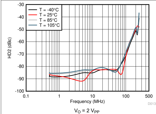
8-15. HD2 vs Frequency Across Temperature
