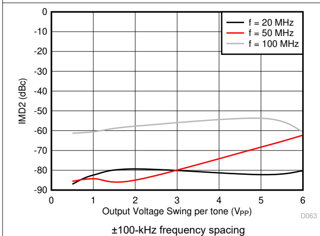
8-52. IMD2 vs Output Voltage Swing
