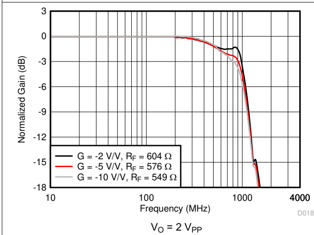
8-3. Inverting Small-Signal Frequency Response
