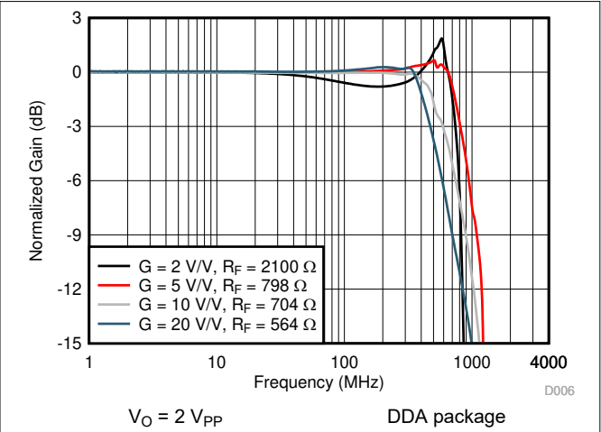
8-2. Noninverting Small-Signal Frequency Response
