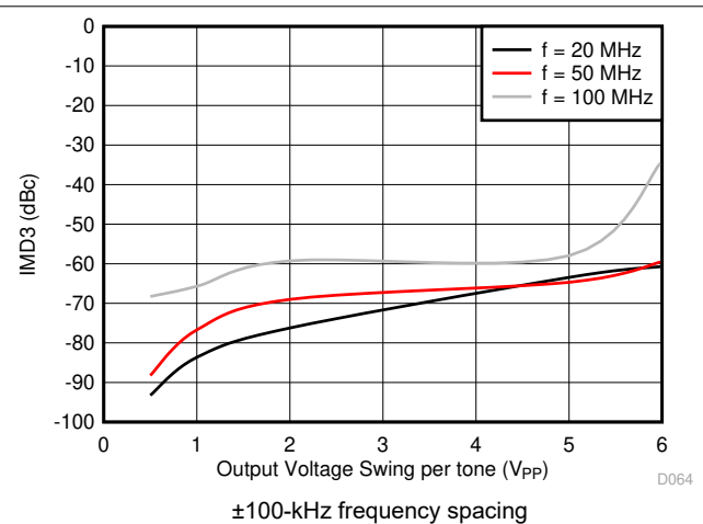
8-53. IMD3 vs Output Voltage Swing
