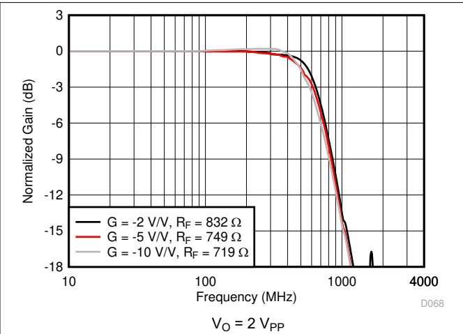
8-43. Inverting Small-Signal Frequency Response
