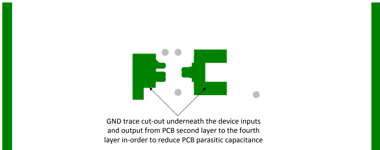
10-13. Ground Trace Cutout Beneath the Device Inputs and Output
