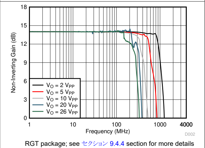
8-4. Frequency Response vs Output Swing
