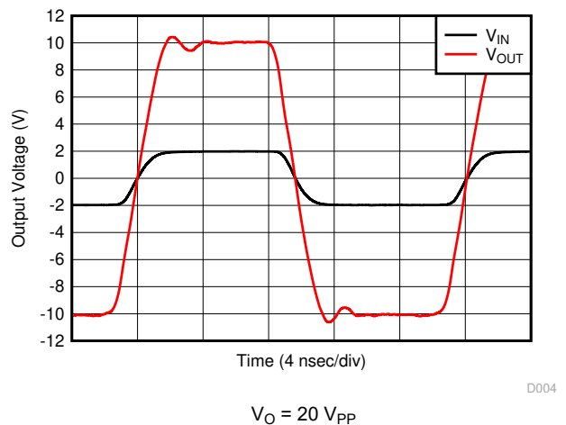
8-24. G = 5 V/V Pulse Response
