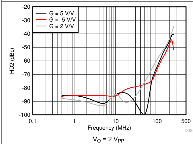
8-44. HD2 vs Frequency
