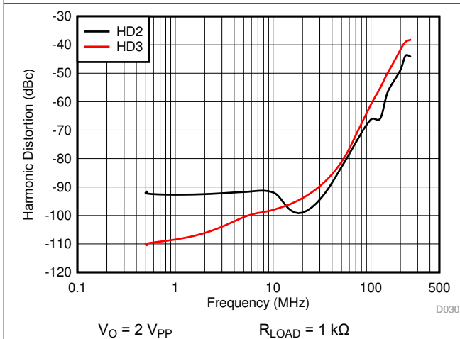
8-50. Harmonic Distortion vs Frequency
