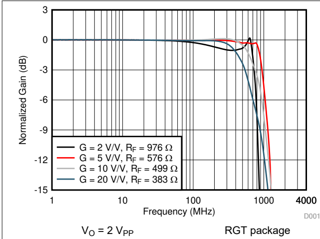
8-1. Noninverting Small-Signal Frequency Response
