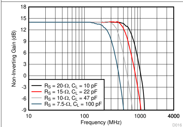
8-5. Frequency Response vs C_{LOAD}
