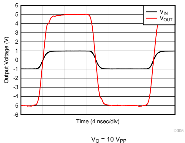
8-23. G = 5 V/V Pulse Response
