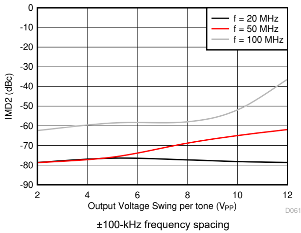
8-19. IMD2 vs Output Voltage Swing
