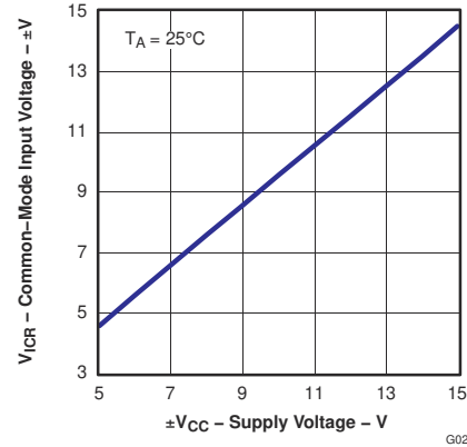
5-51. Common-mode Input Voltage vs Supply Voltage
