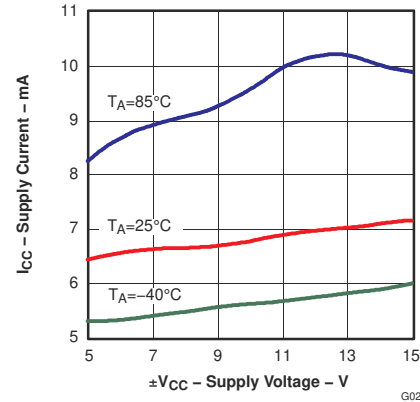
5-53. Supply Current vs Supply Voltage
