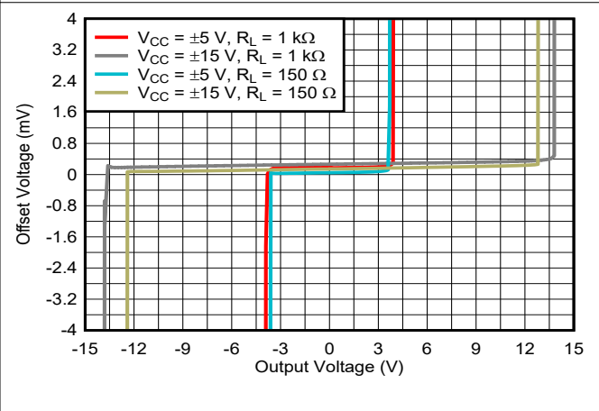
Figure 5-28. Offset Voltage vs Output Voltage
