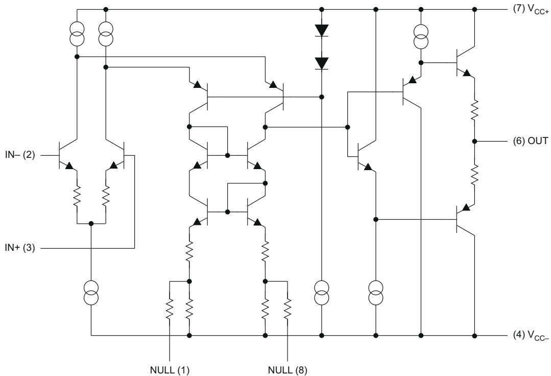
☒ 6-3. THS4021 Simplified Schematic
