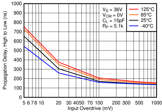
6-32. High to Low Propagation Delay vs. Input Overdrive Voltage, 36V
