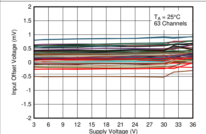
6-15. Input Offset Voltage vs. Supply Voltage at 25^\circ\text{C}
