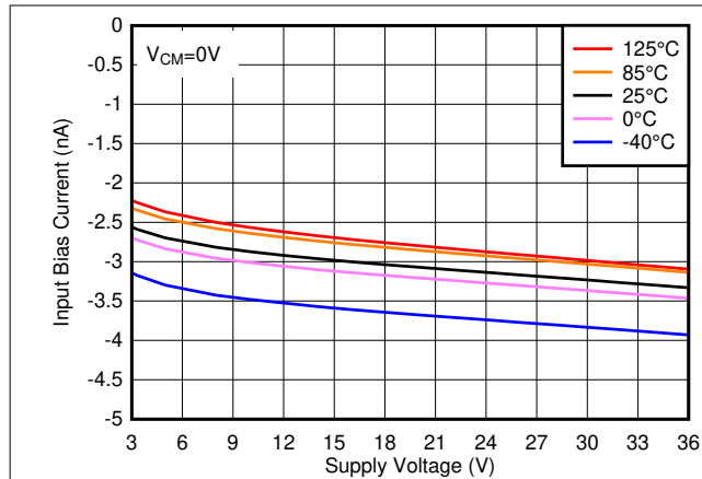
6-10. Input Bias Current vs. Supply Voltage
