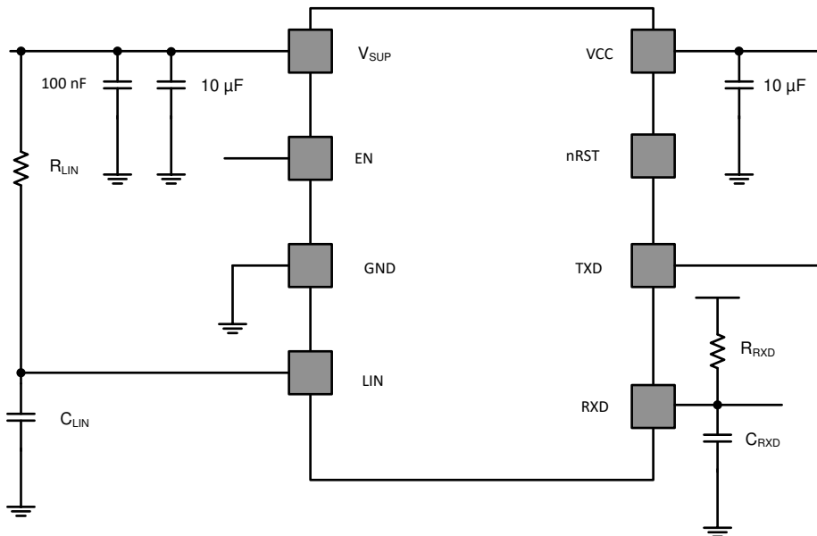
8-17. Test Circuit for AC Characteristics
