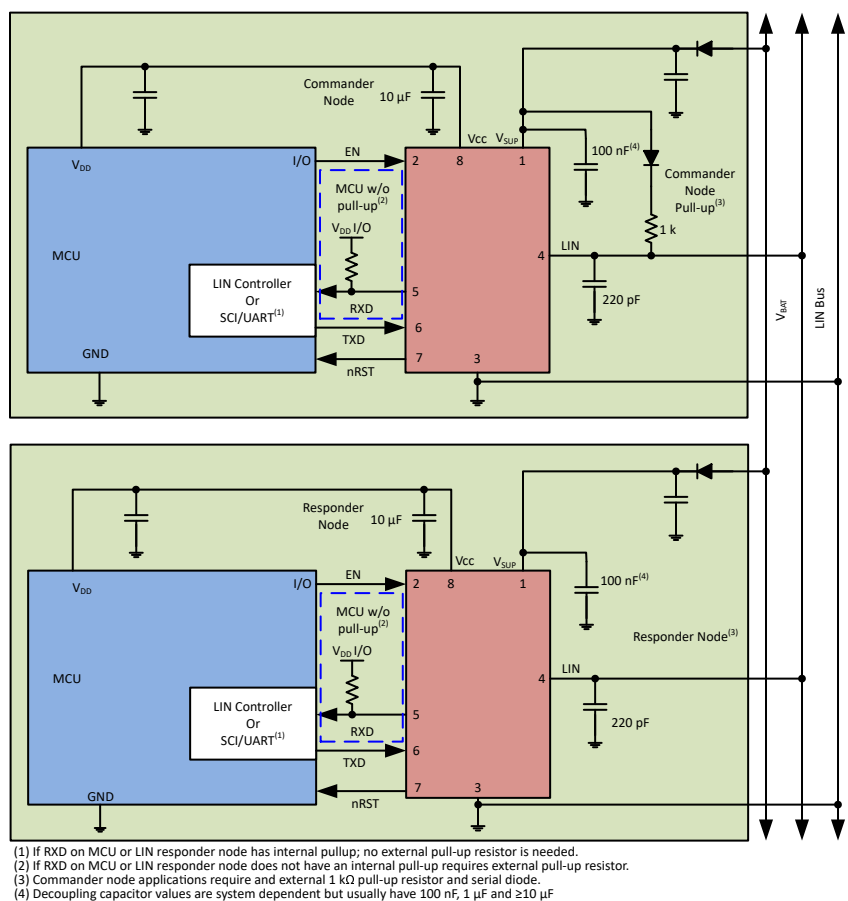
☒ 10-1. Typical LIN Bus
