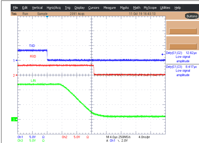
10-8. Recessive to Dominant Propagation Delay
