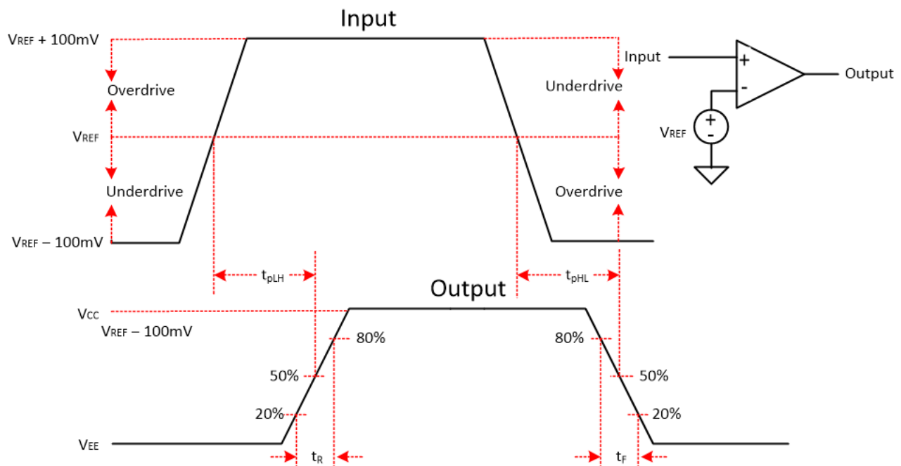
9-1. Comparator Timing Diagram
