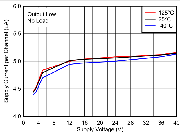
7-1. Supply Current per Channel vs. Supply Voltage, Output Low
