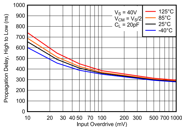
FIG 7-17. Propagation Delay, High to Low, 40 V
