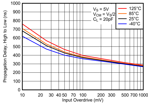
FIG 7-13. Propagation Delay, High to Low, 5 V
