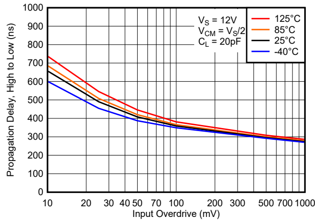
FIG 7-15. Propagation Delay, High to Low, 12 V
