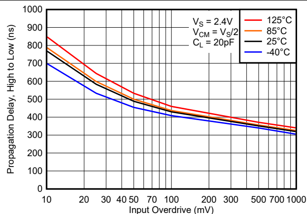
7-11. Propagation Delay, High to Low, 2.4 V
