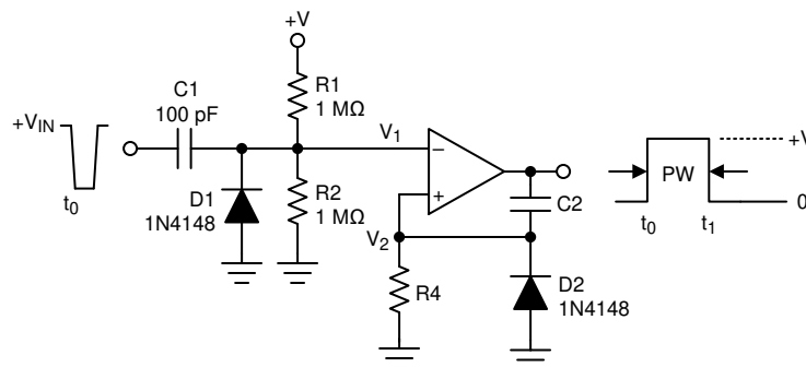
FIG 9-15. One-Shot Multivibrator
