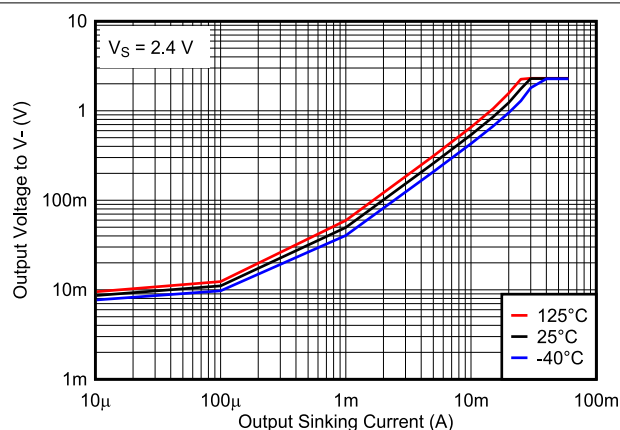
7-3. Output Voltage vs. Output Sinking Current, 2.4 V
