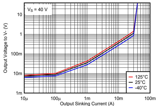
7-9. Output Voltage vs. Output Sinking Current, 40 V
