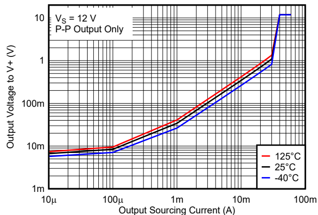
7-8. Output Voltage vs. Output Sourcing Current, 12 V
