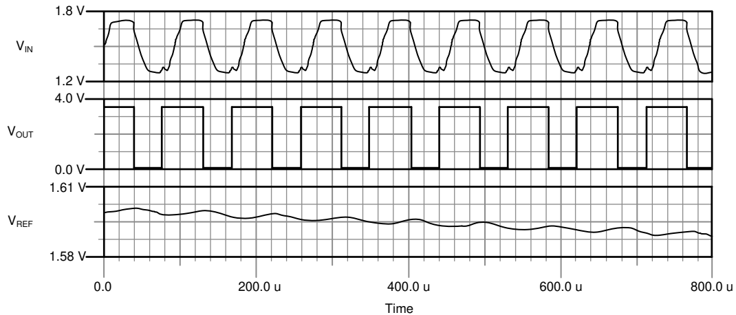
FIG 9-19. Pulse Slicer Waveforms
