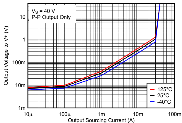
7-10. Output Voltage vs. Output Sourcing Current, 40 V
