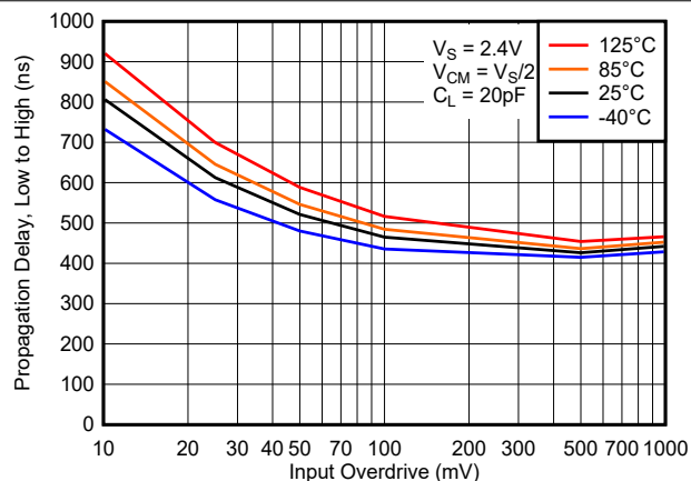
7-12. Propagation Delay, Low to High, 2.4 V
