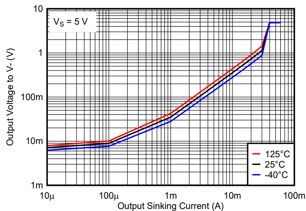
7-5. Output Voltage vs. Output Sinking Current, 5 V
