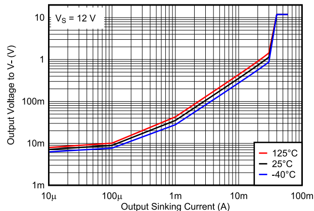
7-7. Output Voltage vs. Output Sinking Current, 12 V
