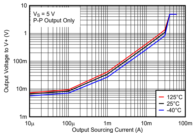
7-6. Output Voltage vs. Output Sourcing Current, 5 V
