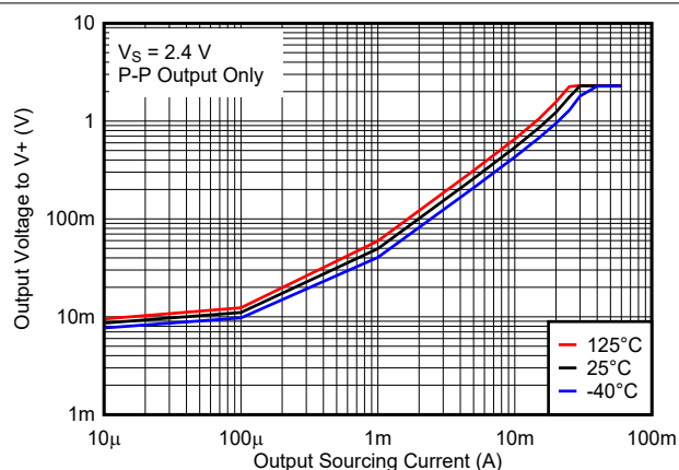
7-4. Output Voltage vs. Output Sourcing Current, 2.4 V
