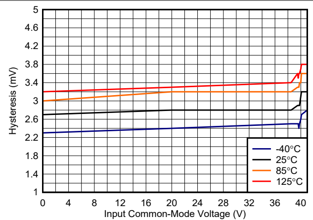
Fig 6-8. Hysteresis vs. Common-Mode, 40 V
