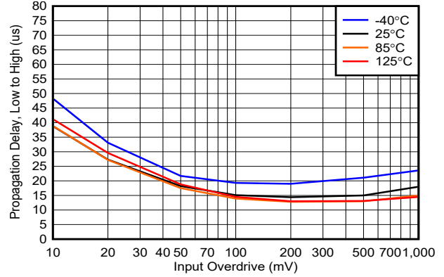
6-32. Propagation Delay, Low to High, 40 V, Push-Pull
