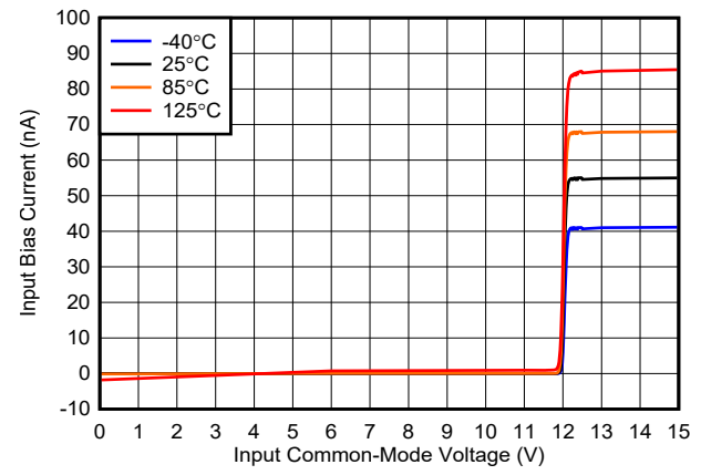
Fig 6-10. Bias Current vs. Common-Mode, 12 V
