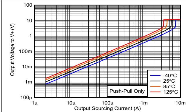
6-15. Output Voltage vs. Output Sourcing Current, 12V
