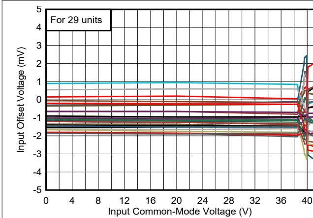
Fig 6-7. Offset vs. Common-Mode, 40 V
