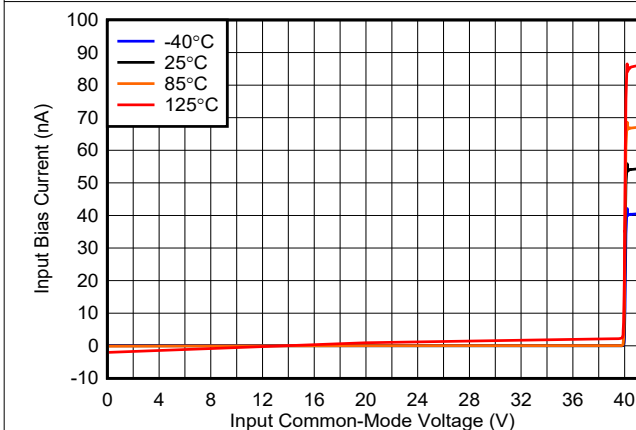
Fig 6-11. Bias Current vs. Common-Mode, 40 V
