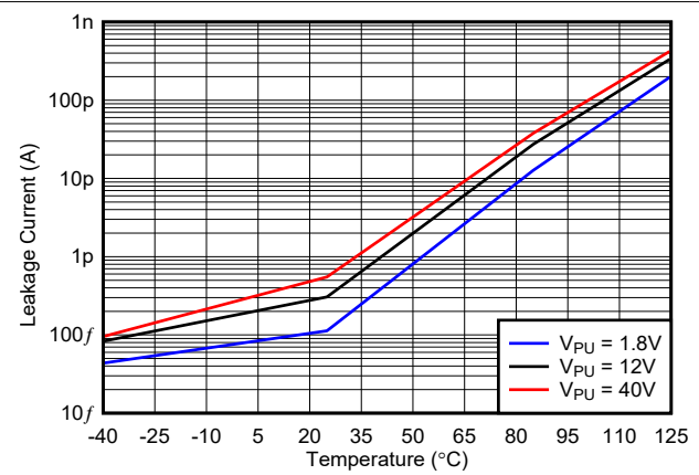
Fig 6-12. Leakage Current vs. Temperature (Open Drain only)
