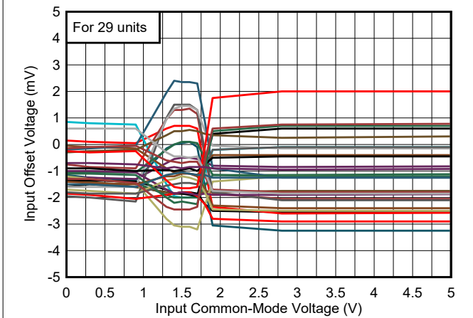
6-3. Offset vs. Common-Mode, 1.8 V
