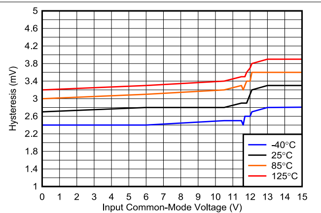
6-6. Hysteresis vs. Common-Mode, 12 V
