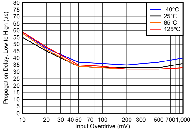
6-31. Propagation Delay, Low to High, 40 V, Open Drain
