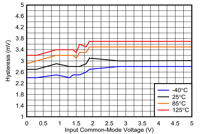
6-4. Hysteresis vs. Common-Mode, 1.8 V
