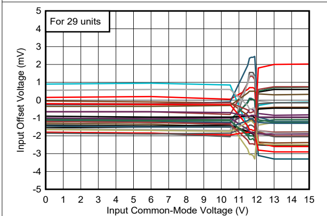
6-5. Offset vs. Common-Mode, 12 V
