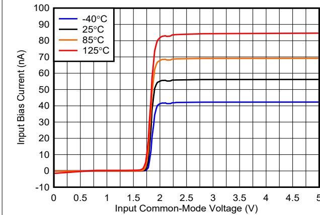
Fig 6-9. Bias Current vs. Common-Mode, 1.8 V
