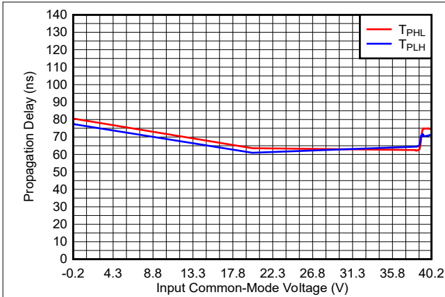
Figure 5-19. Propagation Delay vs. Common-Mode, 40V
