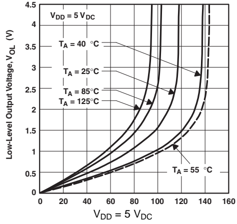
8. Low-level Output Voltage vs Low-Level Output Current
