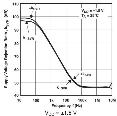
18. Supply-Voltage Rejection Ratio vs Frequency
