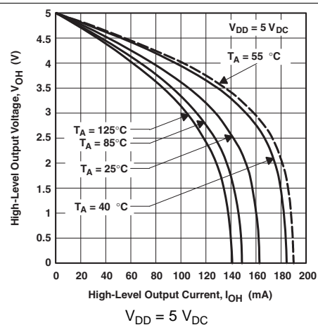
Fig. 6. High-Level Output Voltage vs High-Level Output Current
