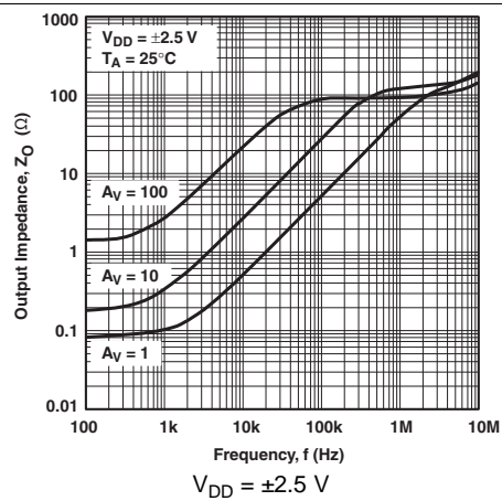
16. Output Impedance vs Frequency
