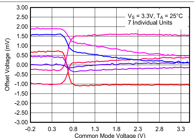
8-30. Offset Voltage vs. Common Mode Voltage, 3.3 V
