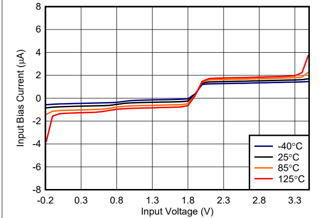
6-23. Bias Current vs. Input Voltage, 3.3 V
