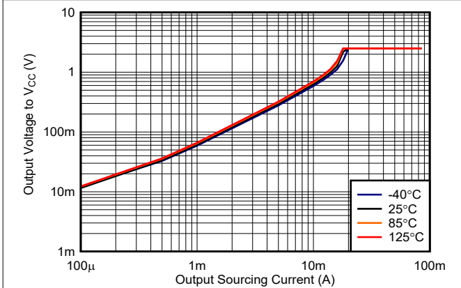
6-25. Output Voltage vs. Output Sourcing Current, 2.5 V
