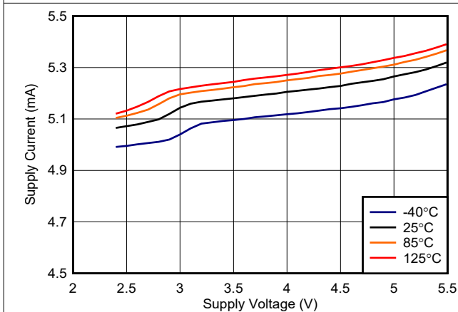
6-31. TLV3601 Supply Current vs. Voltage (Output Low)
