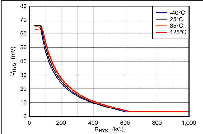
6-21. TLV3603 Hysteresis vs. Resistance, 5 V
