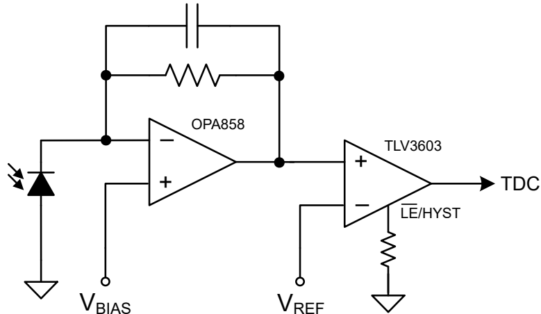
8-9. Optical Receiver
