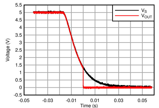
8-4. TLV4041/4051 Output for V_S Falling
