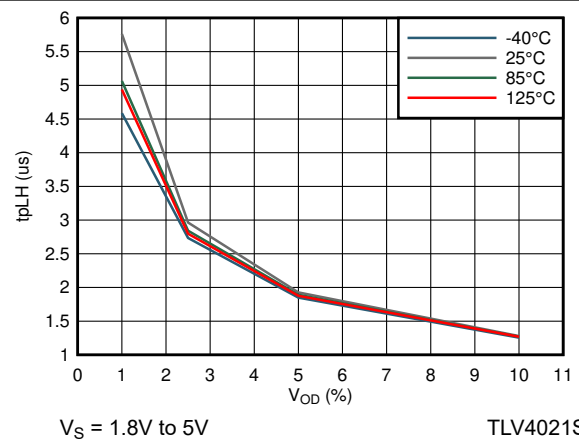
7-30. Propagation Delay Low-High vs Input Overdrive
