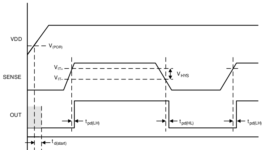
Fig 7-1. Timing Diagram
