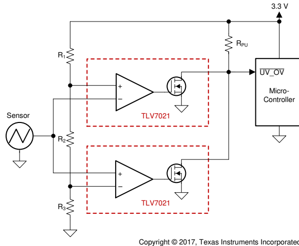
Figure 40. Window Comparator
