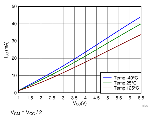
6-20. Output Short Circuit (Sink) vs V_{CC}
