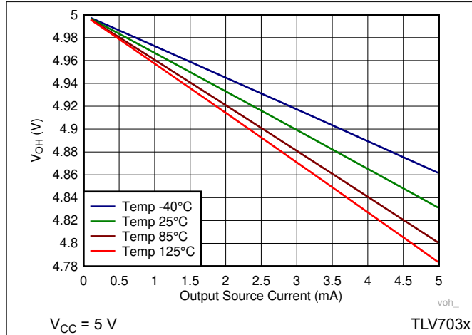
6-15. Output Voltage High vs Output Source Current
