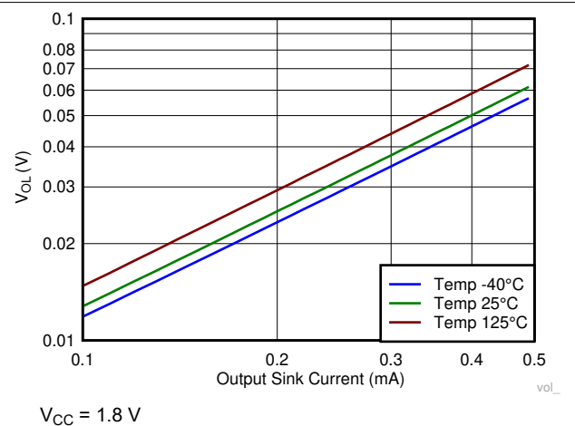
6-16. Output Voltage Low vs Output Sink Current
