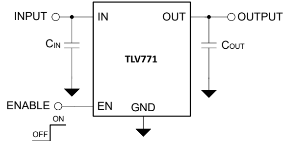
図 7-1. TLV771 Typical Application
