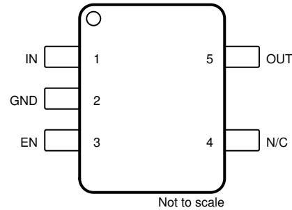
図 4-2. DBV Package, 5-Pin SOT-23 (Top View)
