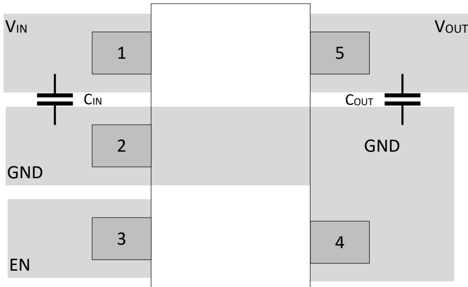
☒ 7-4. DBV Package (SOT-23) Typical Layout
