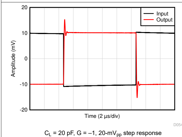
6-35. Small-Signal Step Response
