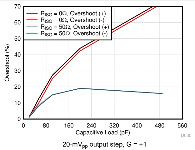
6-32. Small-Signal Overshoot vs Capacitive Load
