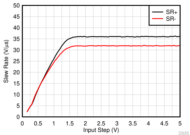
6-15. Slew Rate vs Input Step Voltage
