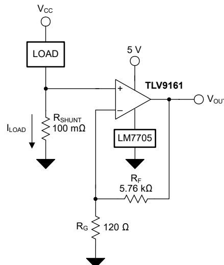
☒ 8-1. TLV9161-Q1 in a Low-Side, Current-Sensing Application
