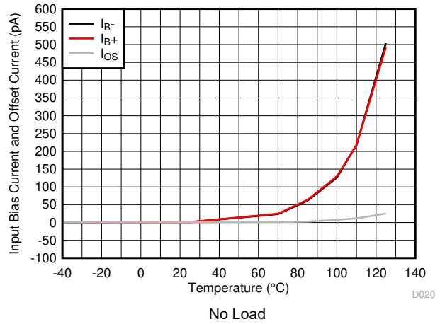
6-14. Input Bias Current and Offset Current vs Temperature
