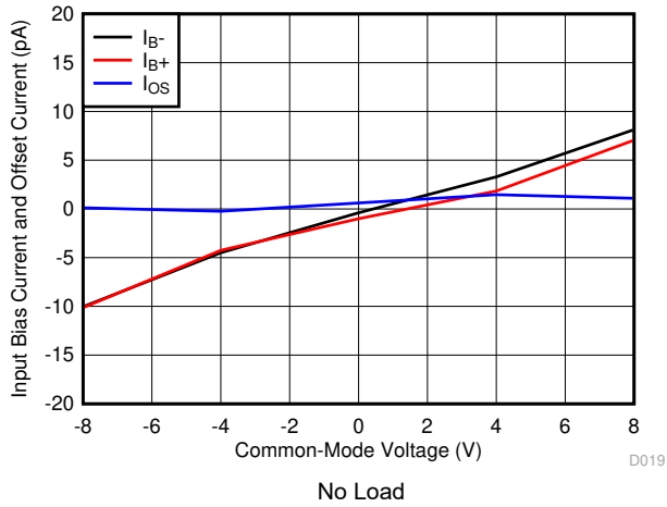
6-13. Input Bias Current and Offset Current vs Common-Mode Voltage
