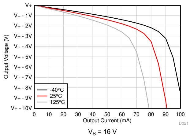
6-16. Output Voltage Swing vs Output Current (Sourcing)
