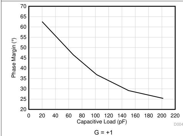
6-33. Phase Margin vs Capacitive Load
