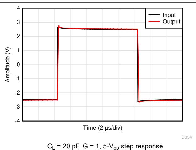
6-36. Large-Signal Step Response
