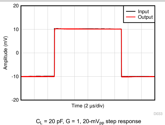
6-34. Small-Signal Step Response
