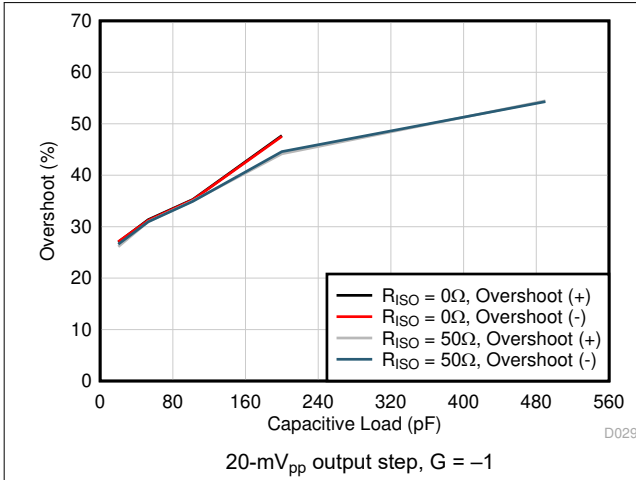
6-31. Small-Signal Overshoot vs Capacitive Load
