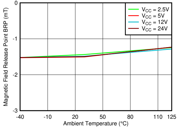
图 7-16. BRP_Y Threshold vs. Temperature
