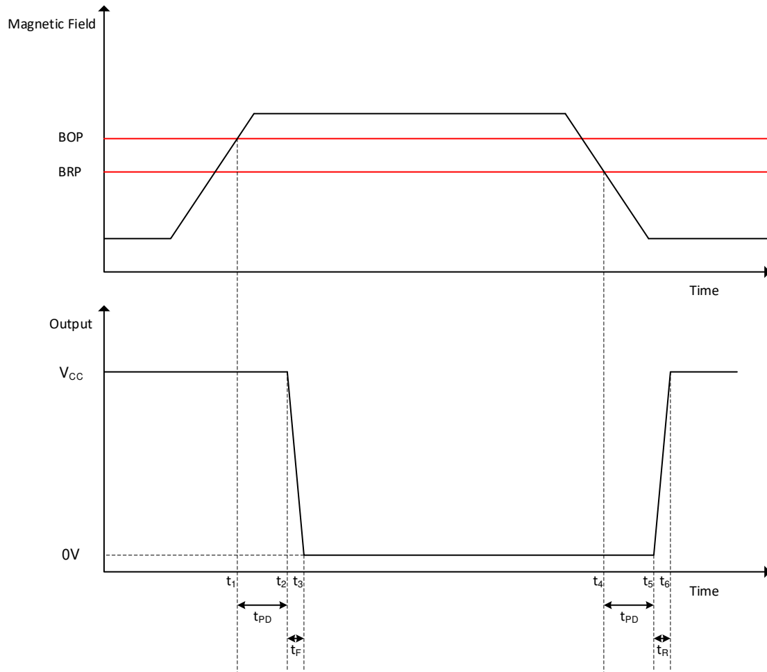
8-20. Propagation Delay
