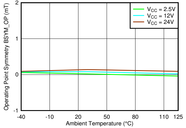
7-64. B_{SYM\_OP(ZX)} vs. Temperature
