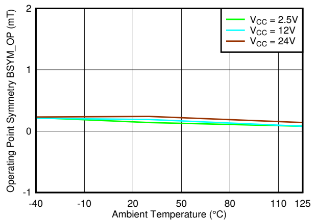
7-68. B_{SYM\_OP(ZY)} vs. Temperature
