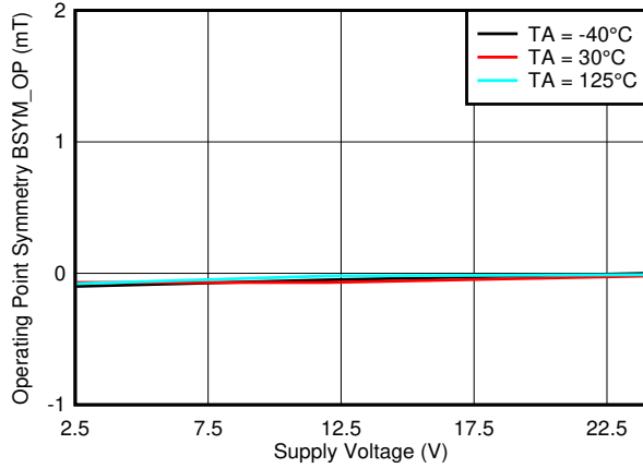
7-33. B_{SYM\_OP(XY)} vs. V_{CC}
