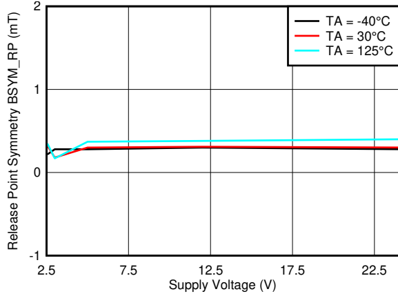
7-31. B_{SYM\_RP(ZY)} vs. V_{CC}
