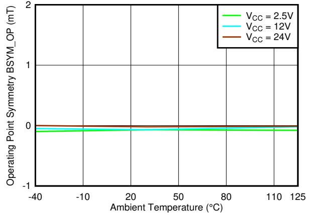
7-34. B_{SYM\_OP(XY)} vs. Temperature
