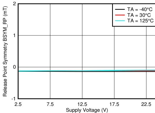
7-35. B_{SYM\_RP(XY)} vs. V_{CC}
