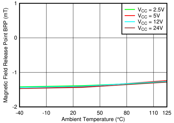
Figure 7-10. B_{RP\_X} Threshold vs. Temperature
