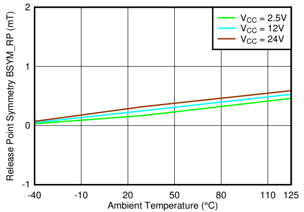
7-66. B_{SYM\_RP(ZX)} vs. Temperature
