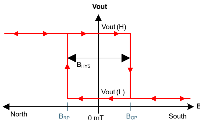
8-2. Latch Functionality
