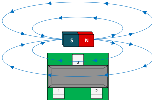
7-4. Positive Magnetic Flux Density: Magnet Offset
