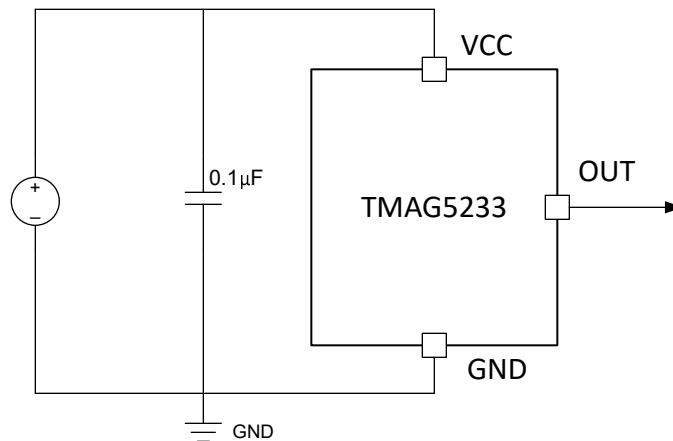
図 8-1. Typical Application Schematic
