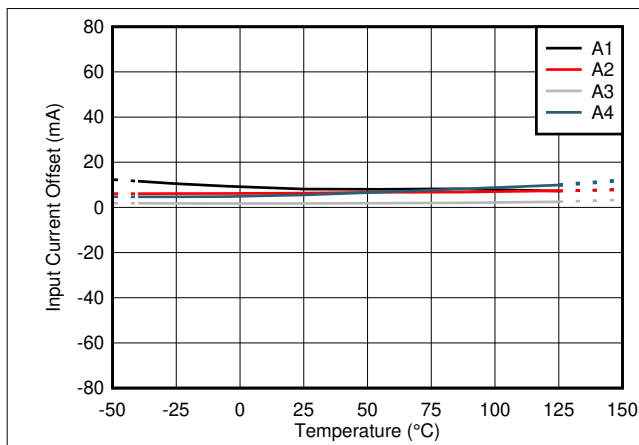
☒ 9-2. Offset Error Drift Across Temperature
