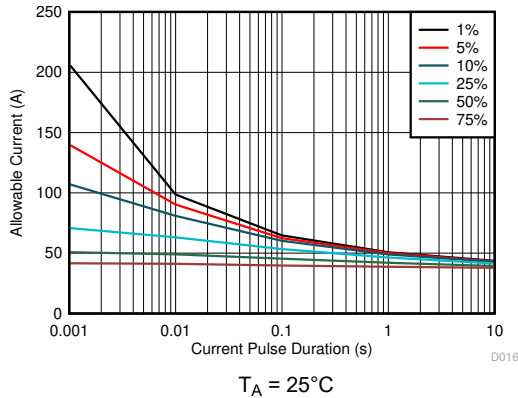
☒ 8-6. Maximum Repetitive Pulsed Current vs. Pulse Duration
