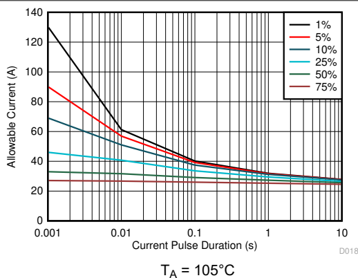
☒ 8-8. Maximum Repetitive Pulsed Current vs. Pulse Duration
