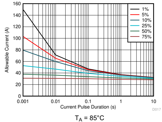
☒ 8-7. Maximum Repetitive Pulsed Current vs. Pulse Duration
