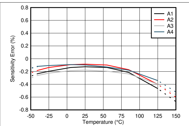
☒ 9-3. Sensitivity Drift Across Temperature
