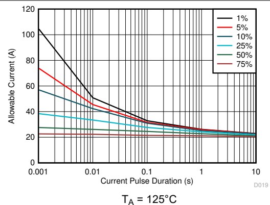
☒ 8-9. Maximum Repetitive Pulsed Current vs. Pulse Duration
