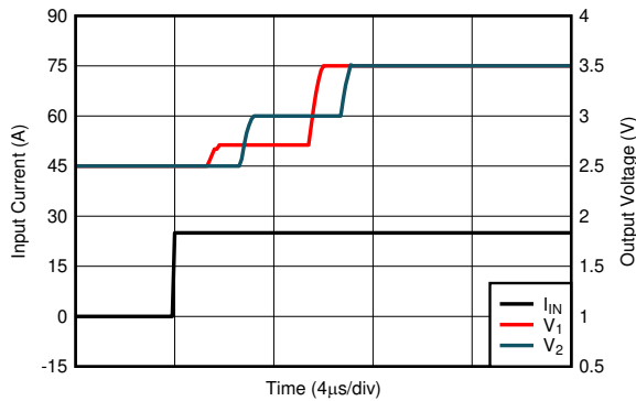
7-17. Voltage Output Step, Rising
