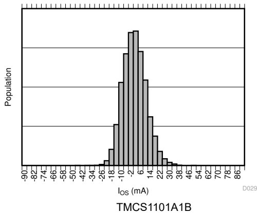
7-9. Input Offset Current Production Distribution
