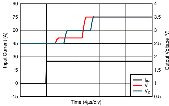
7-23. Voltage Output Step, Rising
