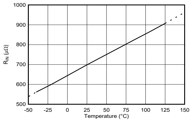
图 6-23. Input Conductor Resistance vs Temperature
