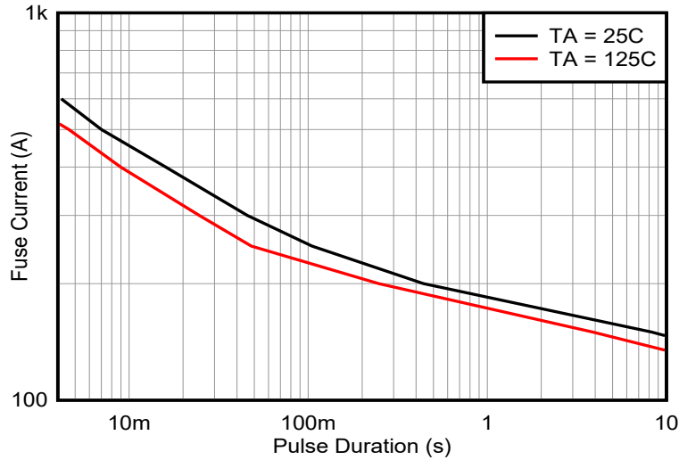
図 7-9. Single-Pulse Leadframe Capability
