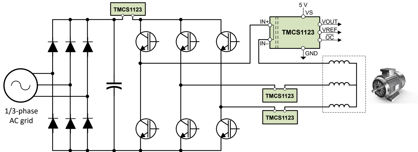
图 9-2. Inline Motor Phase Current Sensing
