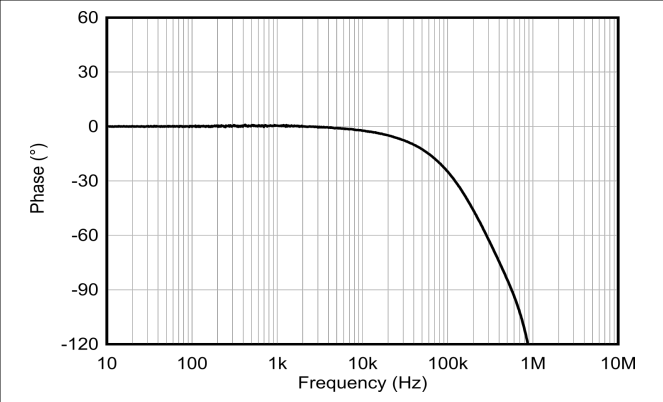
図 6-14. Phase vs Frequency, All Gains
