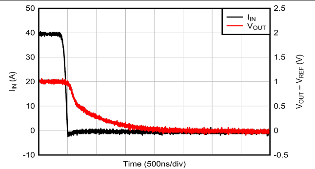
図 6-18. Voltage Output Step Response, Falling
