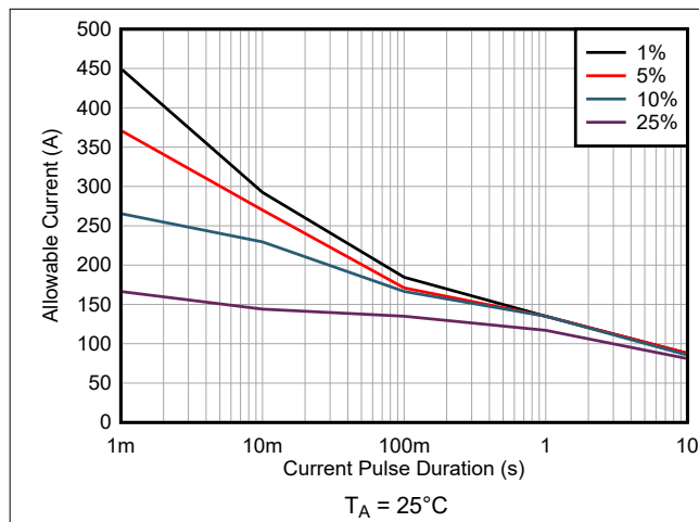
図 7-5. Maximum Repetitive Pulsed Current vs. Pulse Duration
