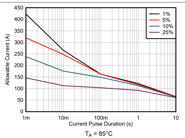
図 7-6. Maximum Repetitive Pulsed Current vs. Pulse Duration
