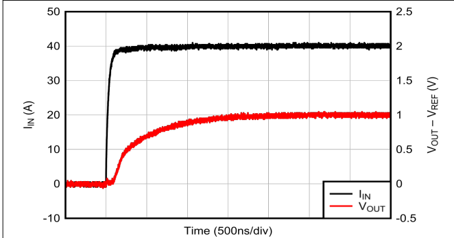
図 6-17. Voltage Output Step Response, Rising
