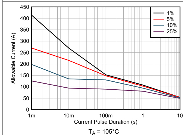
図 7-7. Maximum Repetitive Pulsed Current vs. Pulse Duration
