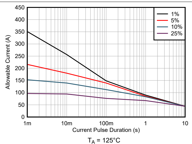
図 7-8. Maximum Repetitive Pulsed Current vs. Pulse Duration
