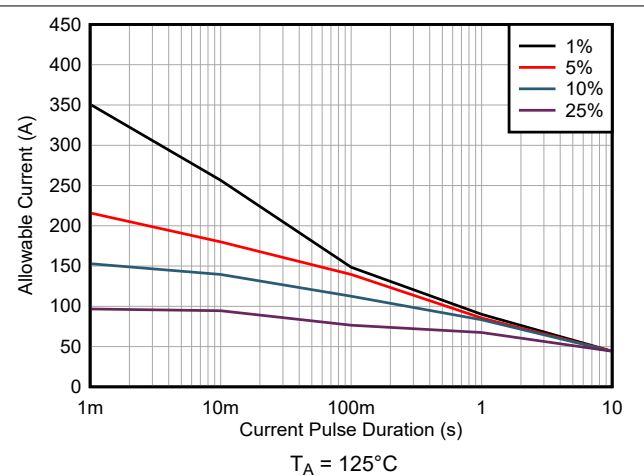
図 7-8. Maximum Repetitive Pulsed Current vs. Pulse Duration
