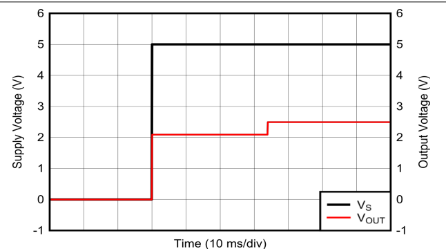
図 6-20. Startup Transient Response
