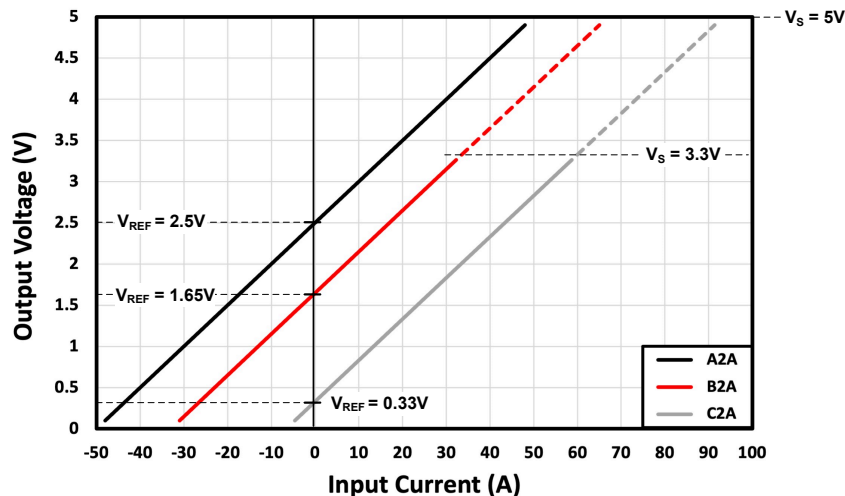
図 8-4. Output Voltage Relationship to Input Current for TMCS1123x2A
