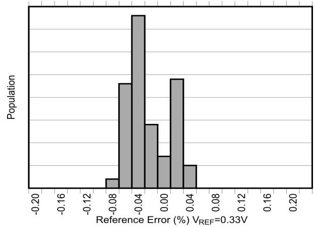
図 6-12. Reference Error Production Distribution
