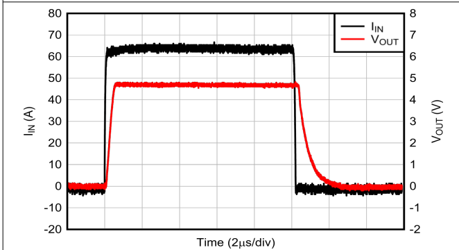
図 6-19. Current Overload Response
