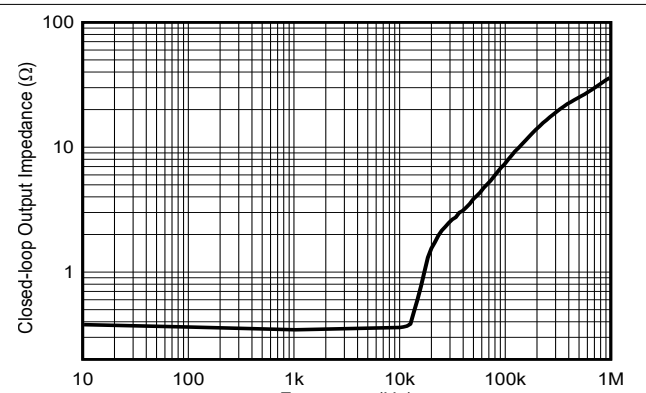
図 6-16. Output Impedance vs Frequency
