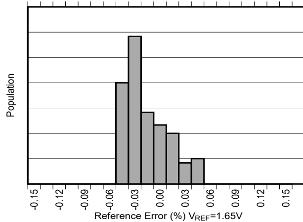
図 6-11. Reference Error Production Distribution
