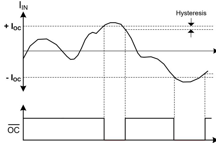
図 8-6. Overcurrent Detection Diagram
