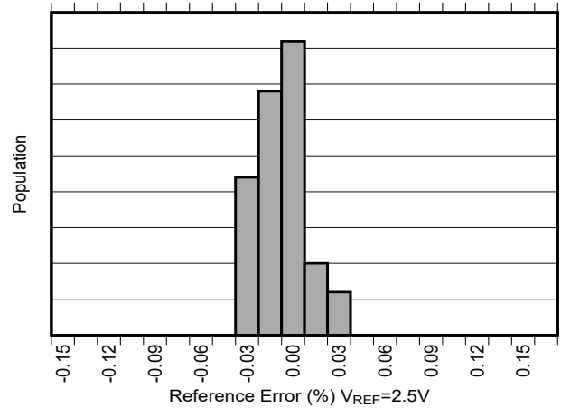
図 6-10. Reference Error Production Distribution
