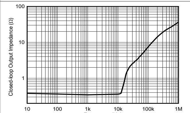
図 6-16. Output Impedance vs Frequency
