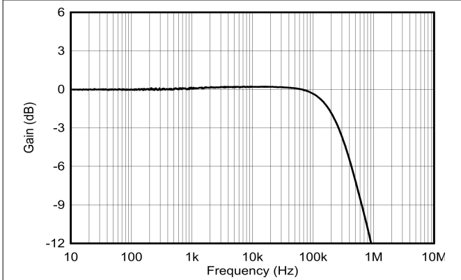
図 6-13. Sensitivity vs Frequency, All Gains Normalized to 1Hz
