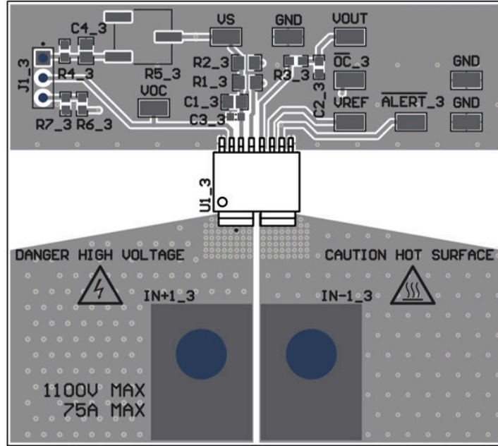
図 9-4. Recommended Board Layout
