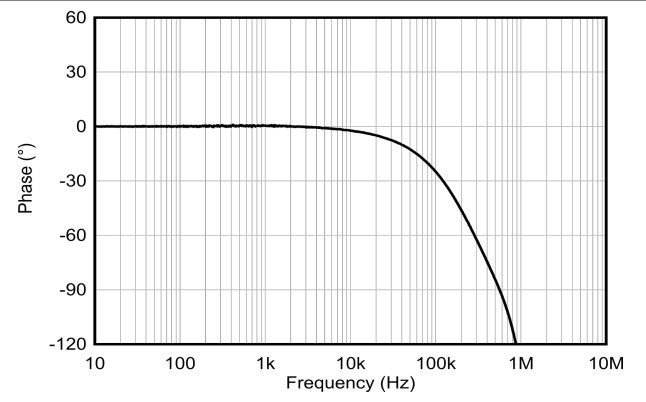
図 6-14. Phase vs Frequency, All Gains
