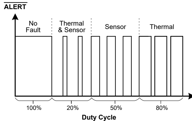
図 8-8. Sensor Diagnostics Waveform
