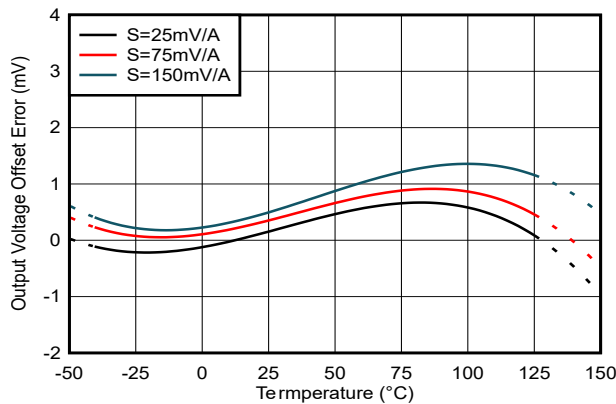
Figure 6-3. Offset Error vs Temperature: TMCS1133Bxx-Q1 Device Options
