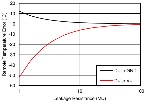
6-4. Remote Temperature Error vs. Leakage Resistance
