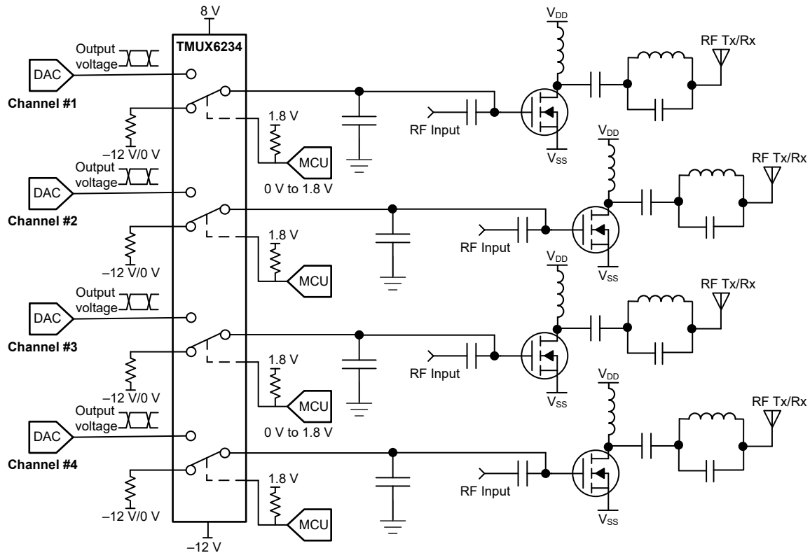
Figure 9-1. Power Amplifier Gate Driver
