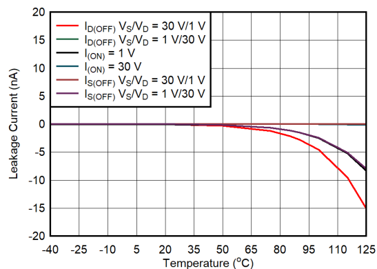
FIG 6-8. Leakage Current vs Temperature
