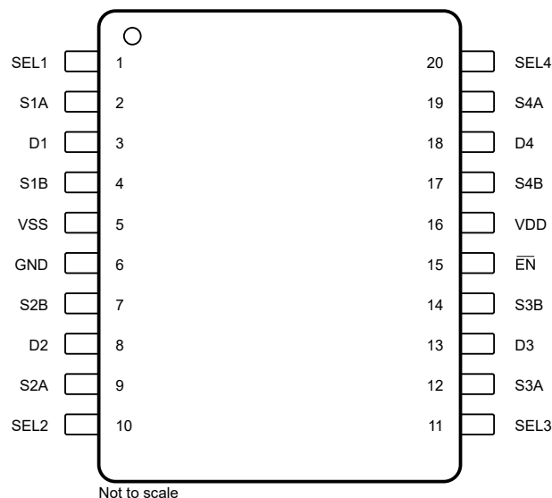
図 5-1. TMUX6234 PW Package, 20-Pin TSSOP (Top View)
