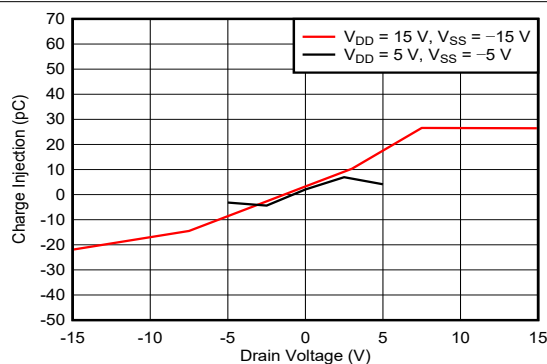
FIG 6-11. Charge Injection vs Source Voltage – Dual Supply
