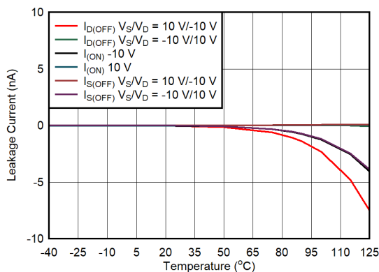
FIG 6-7. Leakage Current vs Temperature
