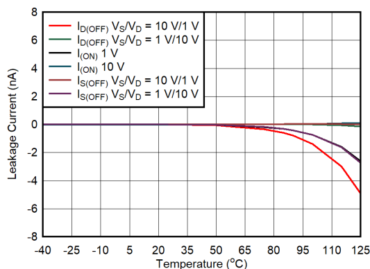
FIG 6-9. Leakage Current vs Temperature
