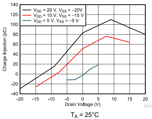
☒ 9-2. Charge Injection vs. Drain Voltage
