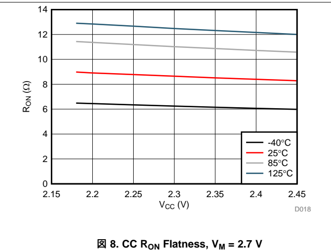
图 8. CC R_{ON} Flatness, V_M = 2.7 V
