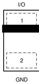
图 5-1. DPY Package 2-Pin X1SON Top View
