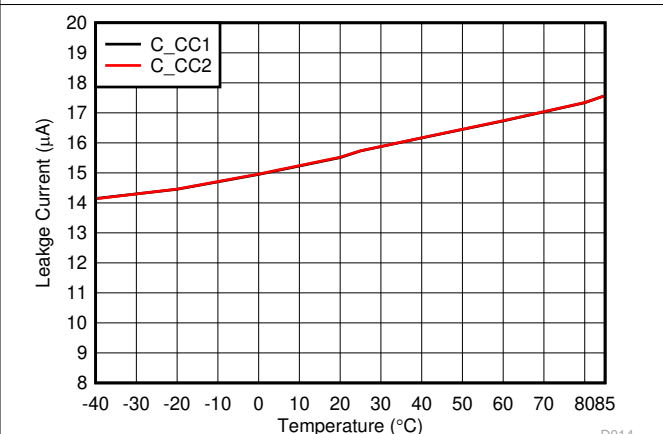
7-24. C CC Path Leakage Current vs Ambient Temperature at C CC = 5.5 V
