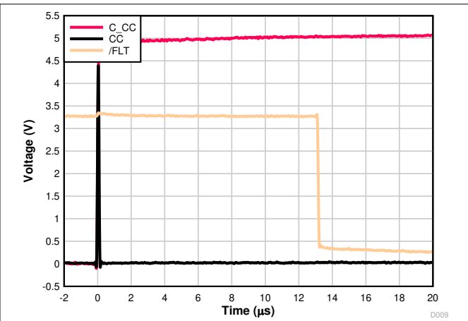
7-20. CC Short-to- V_{BUS} 5 V Zoomed Out
