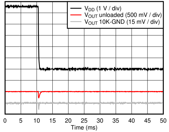
6-40. Power-off Glitch
