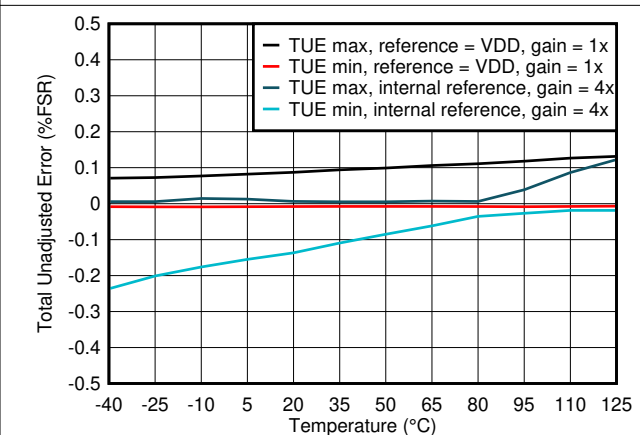
Figure 6-16. Total Unadjusted Error vs Temperature
