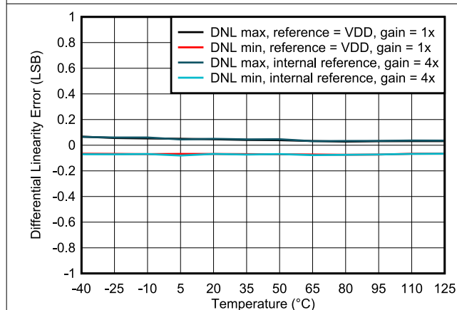
Figure 6-15. Differential Linearity Error vs Temperature
