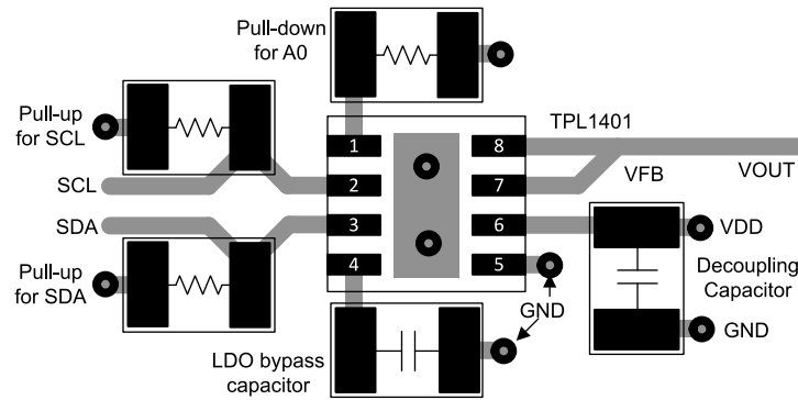
☒ 10-1. Layout Example
