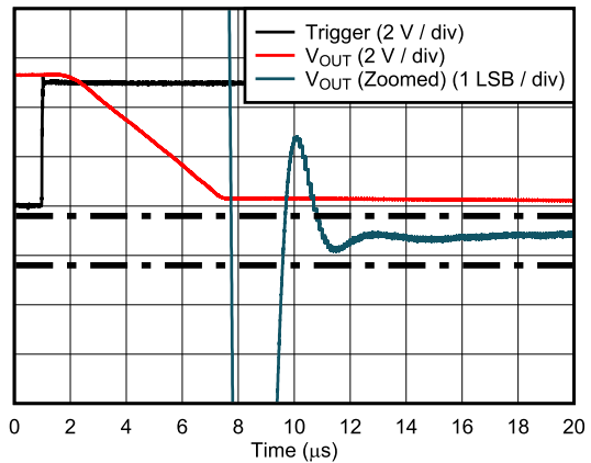
6-36. Glitch Impulse, Falling Edge, 1-LSB Step
