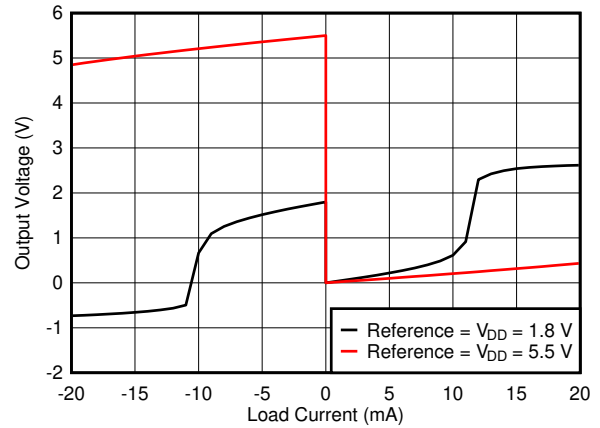
6-34. Source and Sink Capability
