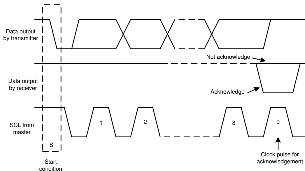
図 7-2. Acknowledge and Not Acknowledge on the I 2 C Bus
