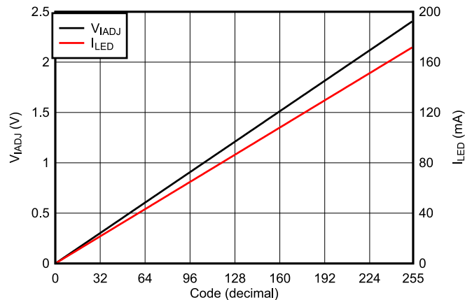
8-2. Digipot Code vs LED Current
