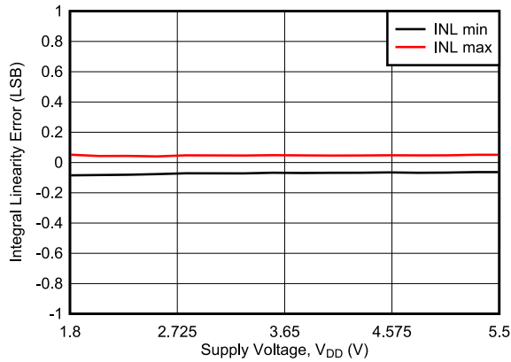
6-21. Integral Linearity Error vs Supply Voltage
