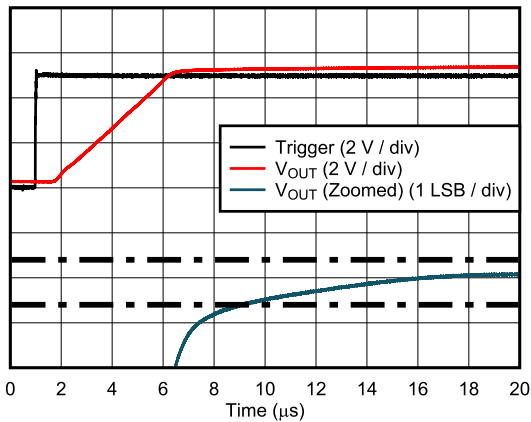
6-35. Glitch Impulse, Rising Edge, 1-LSB Step
