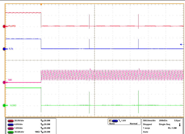
8-7. Auto-Retry Response of TPS1200-Q1 for an Overcurrent Fault
