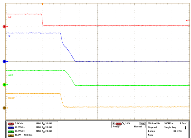
8-5. Turn-OFF Response of TPS1200-Q1 for INP -> HIGH to LOW and C_{BST} = 470 nF
