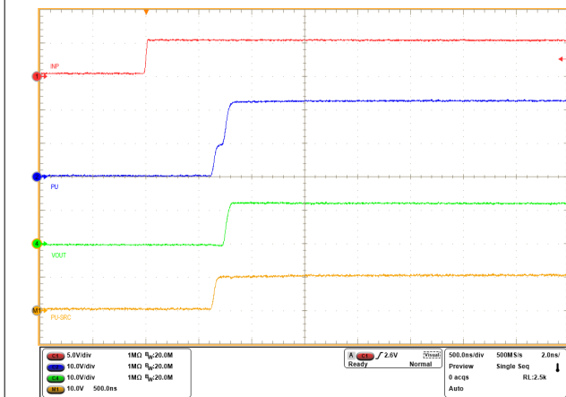
8-4. Turn-ON Response of TPS1200-Q1 for INP -> LOW to HIGH and C_{BST} = 470 nF
