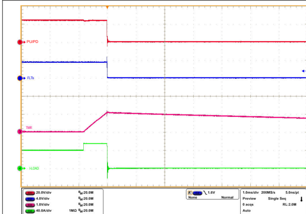
8-6. Overcurrent Response of TPS1200-Q1 for a Load Step from 40 A to 55 A with 50-A Shortcircuit Protection Setting and t_{sc} = 1 ms
