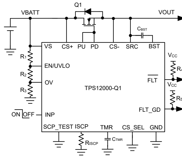
図 8-1. TPS1200-Q1 Application Circuit for driving PAAT loads with VDS based Current Sensing
