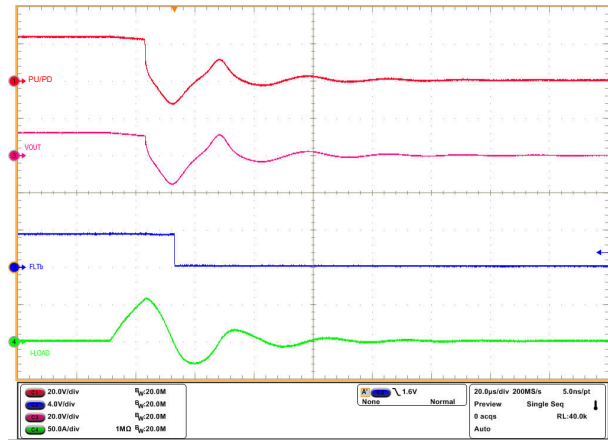
8-9. Output Short-Circuit Response of TPS1200-Q1 Device with 50-A Shortcircuit Protection Setting and TMR = OPEN
