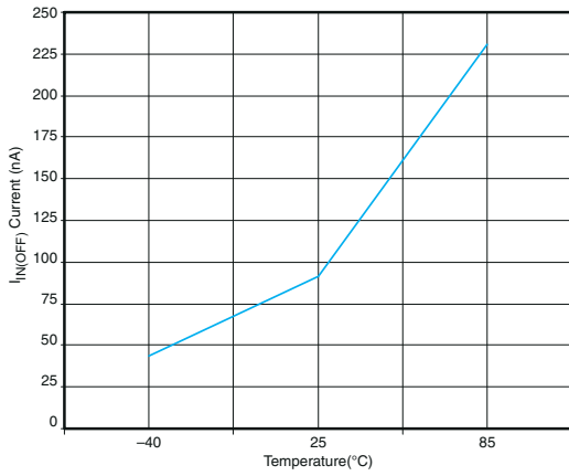
7-7. I_{IN(OFF)} vs Temperature ( V_{IN} = 3.3\text{ V} )
