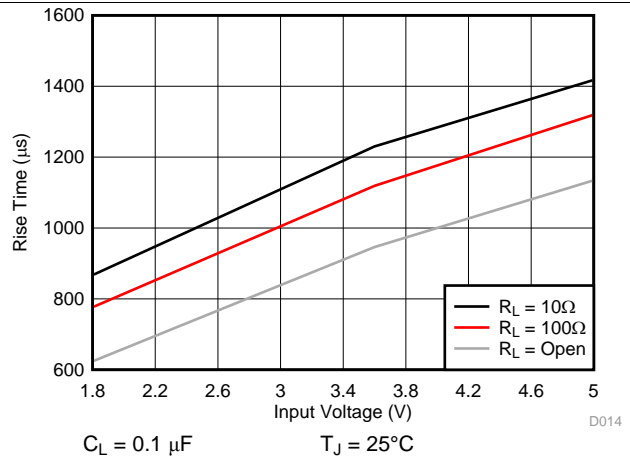
Fig 14. Rise Time vs Input Voltage Across Load Resistance
