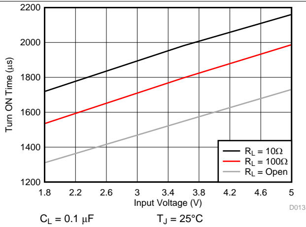
Fig 13. Turn ON Time vs Input Voltage Across Load Resistance
