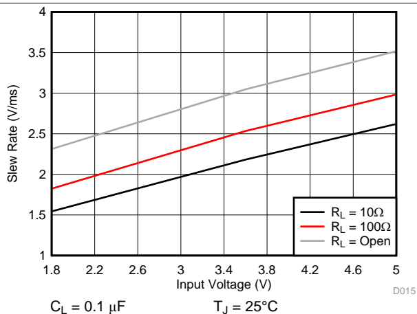
Fig 15. Output Slew Rate vs Input Voltage Across Load Resistance
