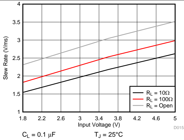
Fig 15. Output Slew Rate vs Input Voltage Across Load Resistance
