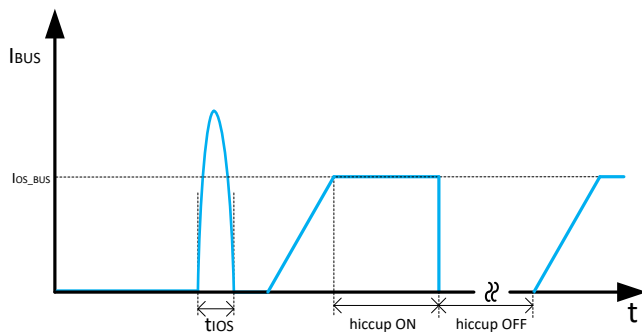
10-11. Response Time to BUS Short-Circuit
