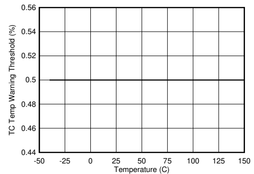
8-22. TS Temperature Warning Threshold vs Junction Temperature
