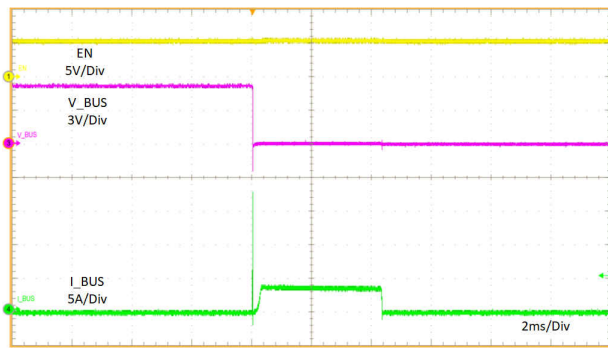
11-24. VBUS Hot Short to GND
