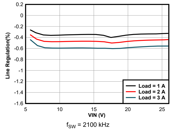
11-7. Line Regulation
