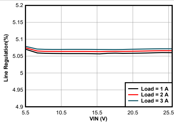
11-12. Dropout Characteristic
