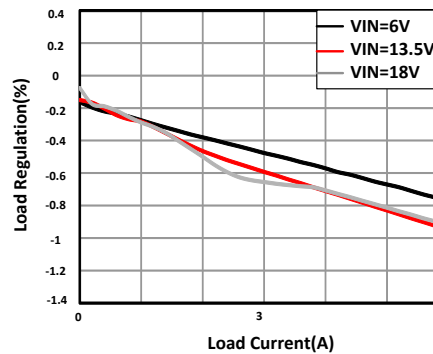
11-6. Load Regulation
