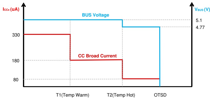
10-17. TPS2586x-Q1 Behavior When Trigger Temp Warm/Hot Threshold
