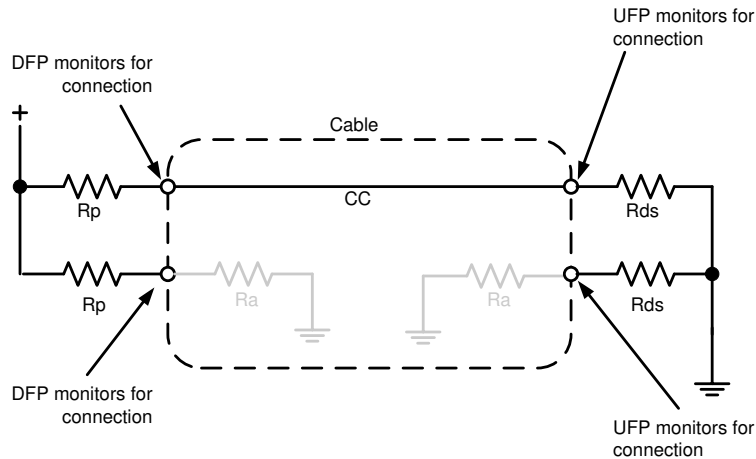
10-20. DFP-UFP Connection
