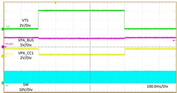
11-30. OUT Hot Short to GND
