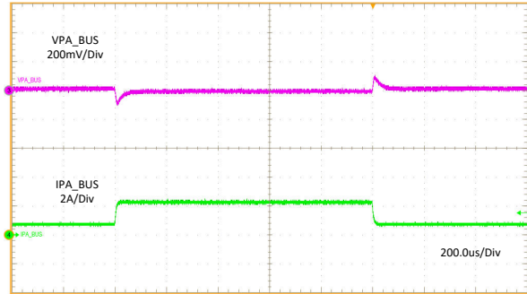
11-10. Load Transient Without Cable Compensation
