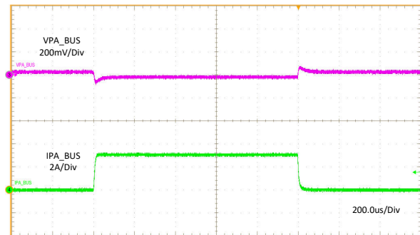
11-6. Load Regulation
