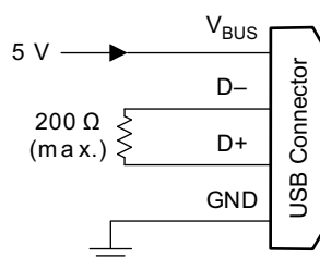
Figure 10-22. DCP Supporting BC1.2 and YD/T 1591-2009
