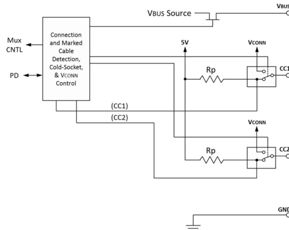
Figure 10-21. Source Functional Model for CC1 and CC2 (From Type-C Specification)
