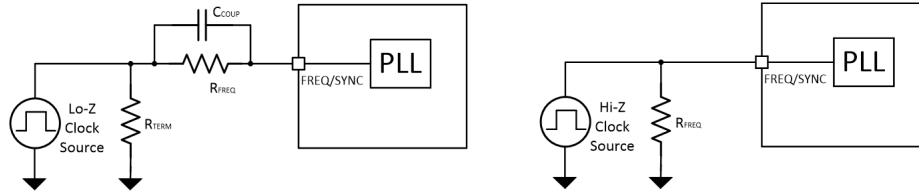
10-4. Synchronize to External Clock
