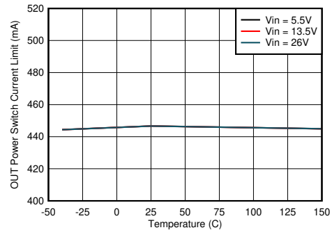
8-14. OUT Power Switch Current Limit vs Junction Temperature
