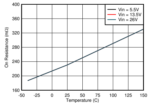
8-18. OUT Power Switch On Resistance vs Junction Temperature
