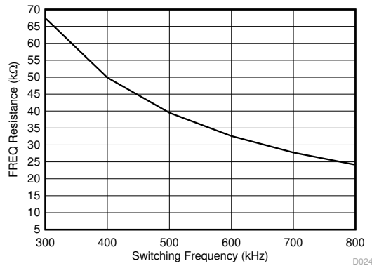
图 10-3. FREQ Set Resistor vs Switching Frequency
