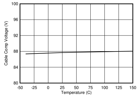
8-16. Cable Compensation Voltage vs Junction Temperature
