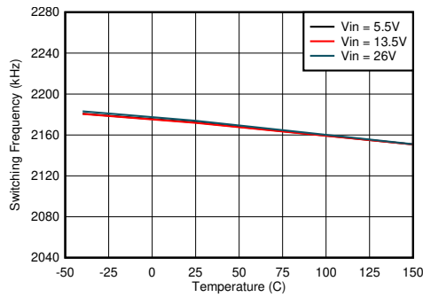
8-21. Switching Frequency vs Junction Temperature
