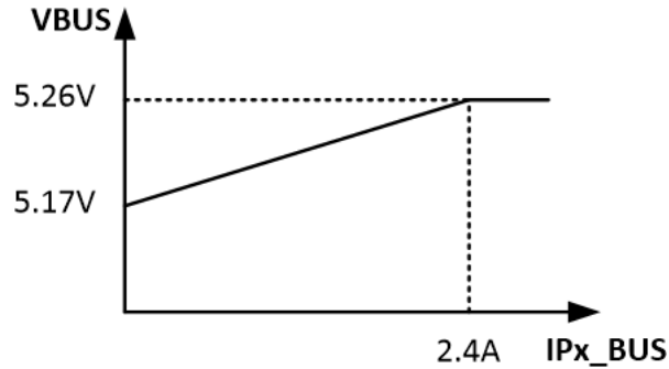
10-9. Dual Ports Cable Compensation
