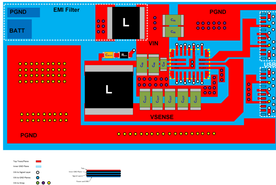
13-1. Layout Example
