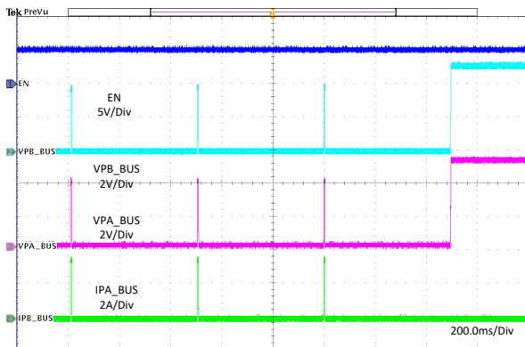
11-25. 1- \Omega Load Recovery
