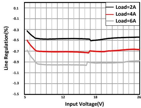
11-6. Line Regulation
