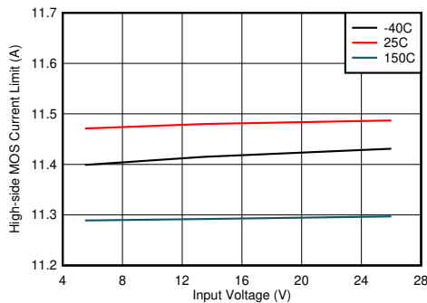
8-7. High-side Current Limit vs Input Voltage
