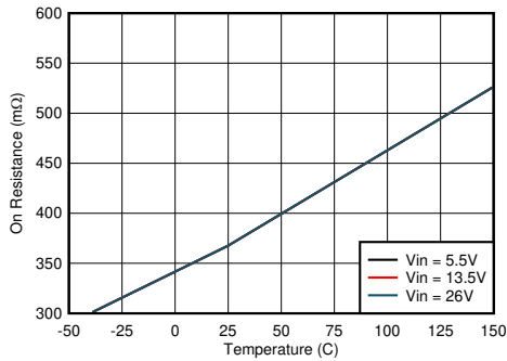
8-19. V_{CONN} Power Switch On Resistance vs Junction Temperature
