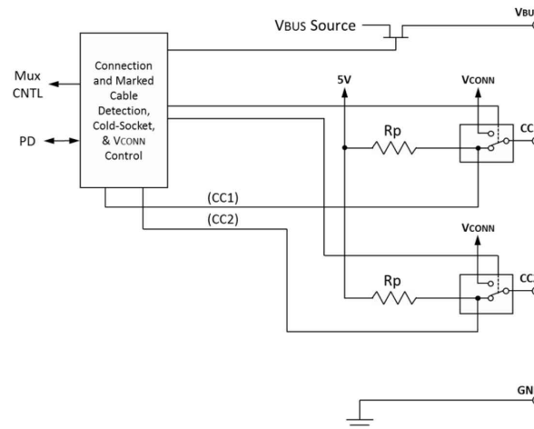
10-15. Source Functional Model for CC1 and CC2 (From Type-C Specification)
