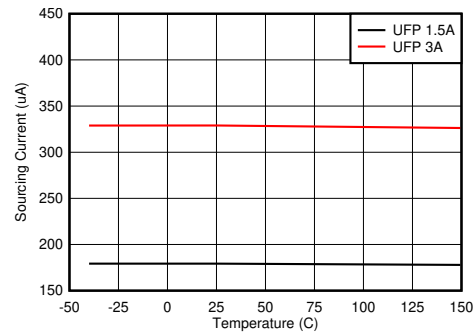
8-22. CC Sourcing Current vs Junction Temperature
