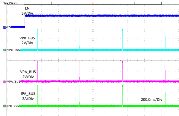
11-22. Enable Into Short
