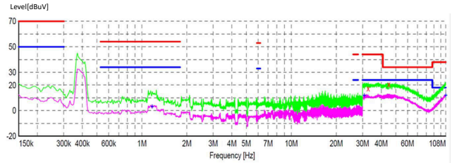
11-4. 400-kHz EMI Results (Without CM Filter)
