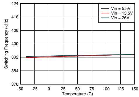
8-20. Switching Frequency vs Junction Temperature
