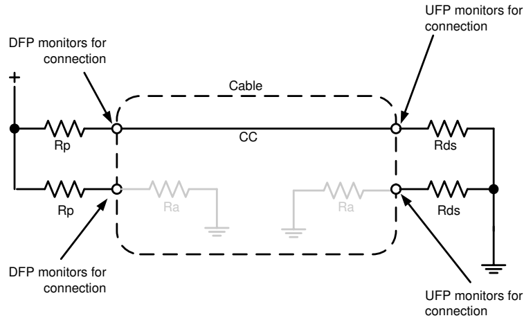
10-14. DFP-UFP Connection
