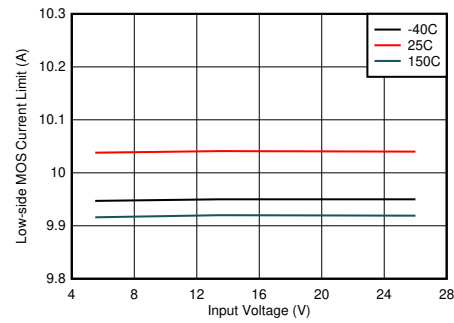
8-8. Low-side Current Limit vs Input Voltage
