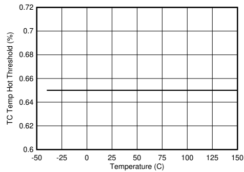
8-24. TS Temperature Hot Threshold vs Junction Temperature
