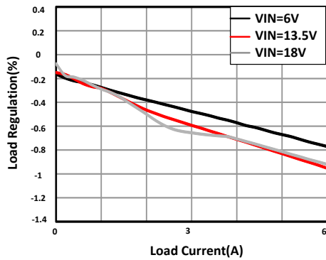
11-5. Load Regulation
