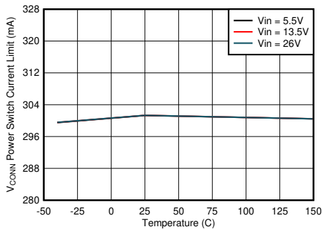
8-15. VCONN Power Switch Current Limit vs Junction Temperature
