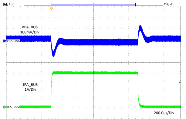
11-5. Load Regulation
