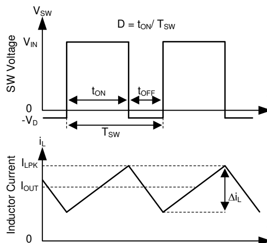
Fig 10-2. SW Node and Inductor Current Waveforms in Continuous Conduction Mode (CCM)
