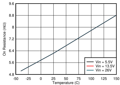
8-17. USB Power Switch On Resistance vs Junction Temperature
