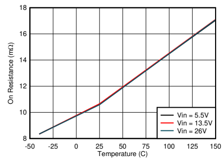
8-10. Low-side MOSFET on Resistance vs Junction Temperature
