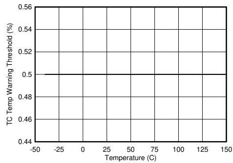
8-23. TS Temperature Wam Threshold vs Junction Temperature
