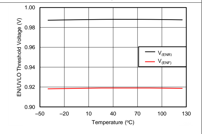
Figure 4. EN Threshold Voltage vs Temperature
