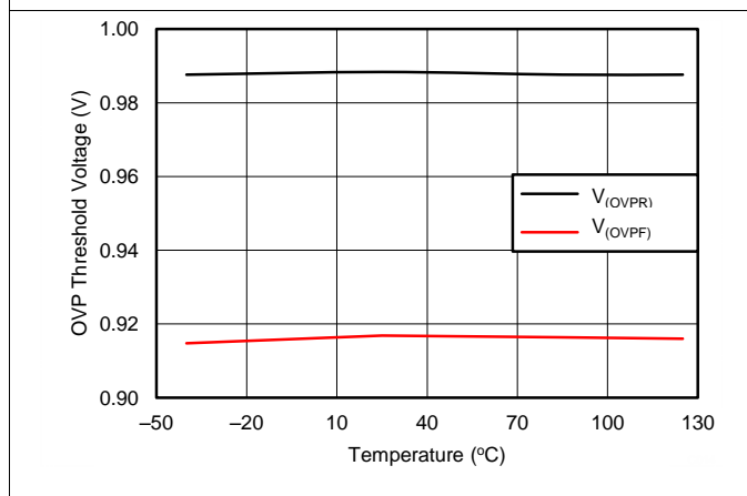
Figure 5. OVP Threshold Voltage vs Temperature
