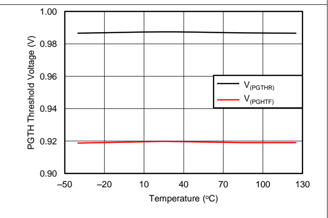
Figure 6. PGTH Threshold Voltage vs Temperature
