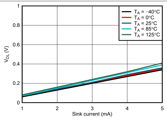
7-11. WDO V_{OL} vs I_{sink} , V_{DD} = 1.5\text{ V}
