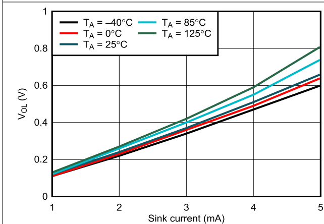
7-10. RESET V_{OL} vs I_{sink} , V_{DD} = 1.5\text{ V}
