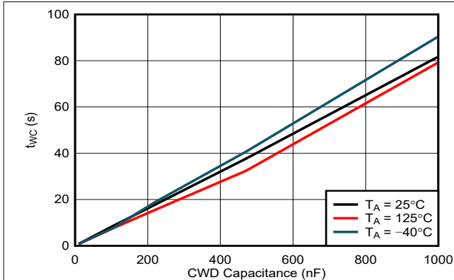
7-8. t_{wc} vs Capacitance
