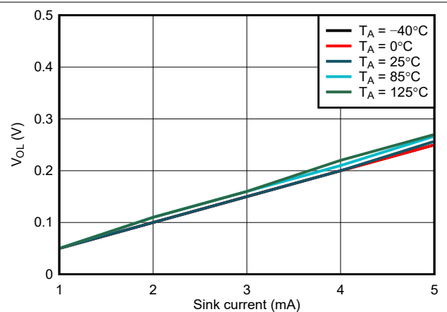
7-13. WDO V_{OL} vs I_{sink} , V_{DD} = 3.3\text{ V}
