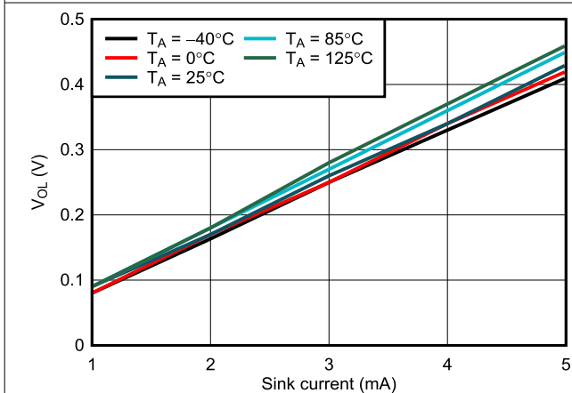
7-12. RESET V_{OL} vs I_{sink} , V_{DD} = 3.3\text{ V}
