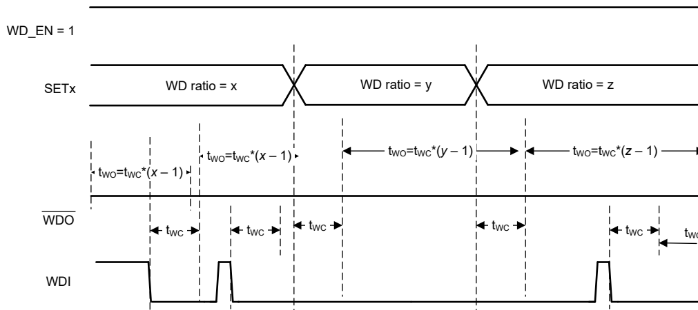
図 8-9. Watchdog Behavior with SETx Pin Status
