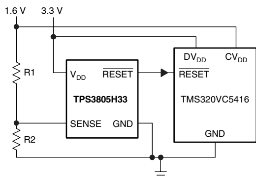
Typical Operating Circuit
