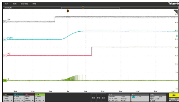
图 8-6. Start-Up Relative to EN Rising, Iout = 0A, PSM Mode
