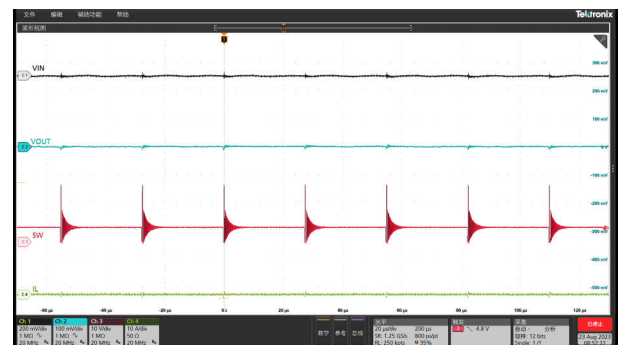
8-13. Output Voltage Ripple, Iout = 0 A, OOA Mode
