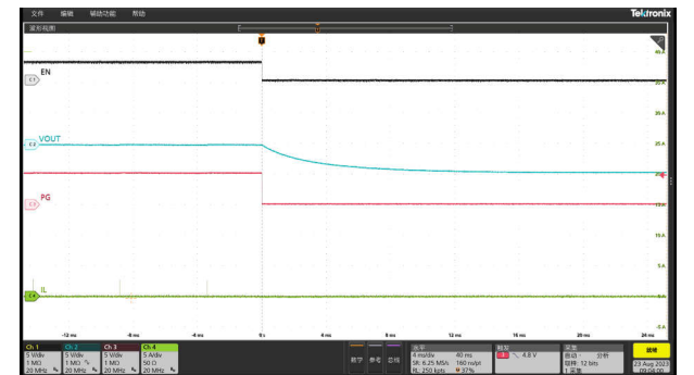
图 8-7. Shutdown Relative to EN Falling, Iout = 0A, PSM Mode
