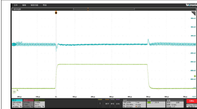
8-16. Transient Response, 0.7 A to 6.3 A with 2.5 A/us SR
