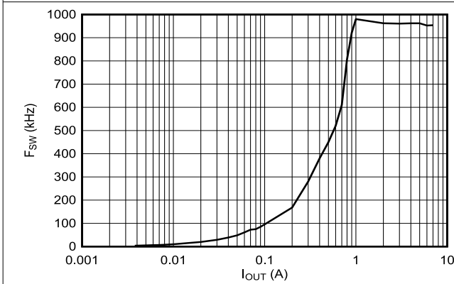
图 8-4. Switching Frequency, PSM Mode
