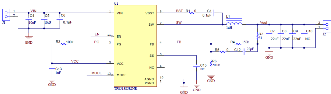
图 8-1. Application Schematic
