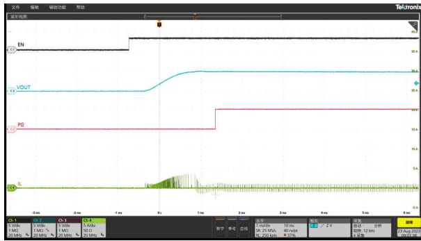
8-8. Start-Up Relative to EN Rising, Iout = 0A, OOA Mode
