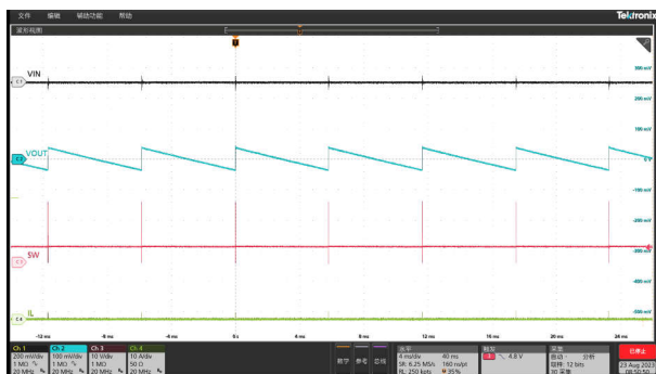
8-12. Output Voltage Ripple, Iout = 0 A, PSM Mode
