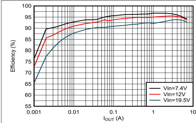
图 8-2. Efficiency, PSM Mode
