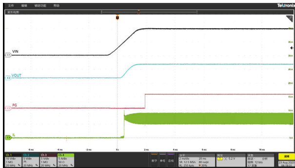
8-10. Start-Up Relative to Vin Rising, Iout = 7A
