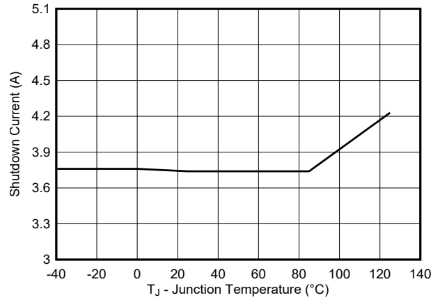
图 6-2. Shutdown Current vs Temperature
