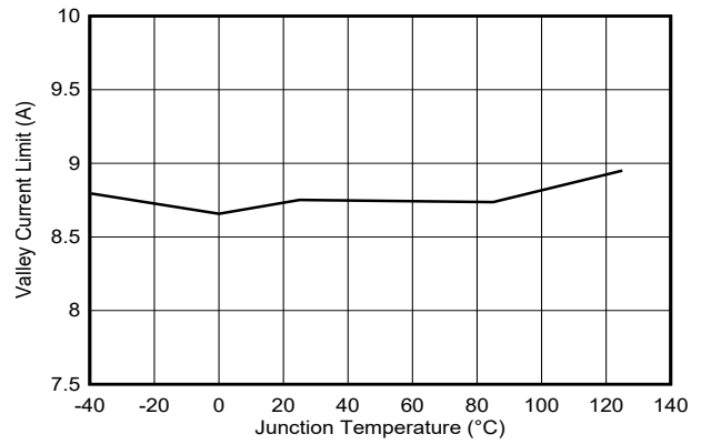
Figure 6-8. Valley Current Limit vs Temperature
