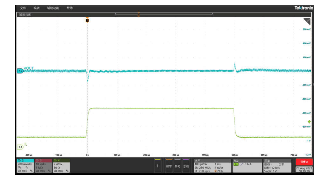
8-15. Transient Response, 1.4 A to 5.6 A with 2.5 A/us SR
