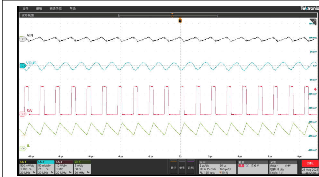
8-14. Output Voltage Ripple, I_{out} = 7\text{ A}
