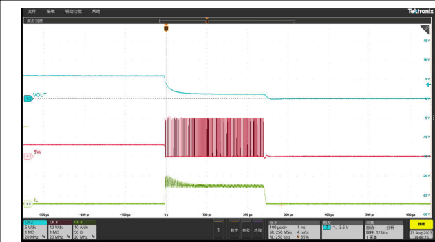
8-17. Normal Operation to Output Hard Short
