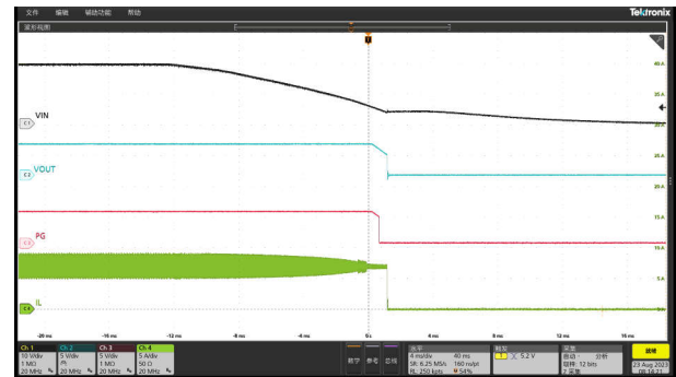
8-11. Shutdown Relative to Vin Falling, Iout = 7A
