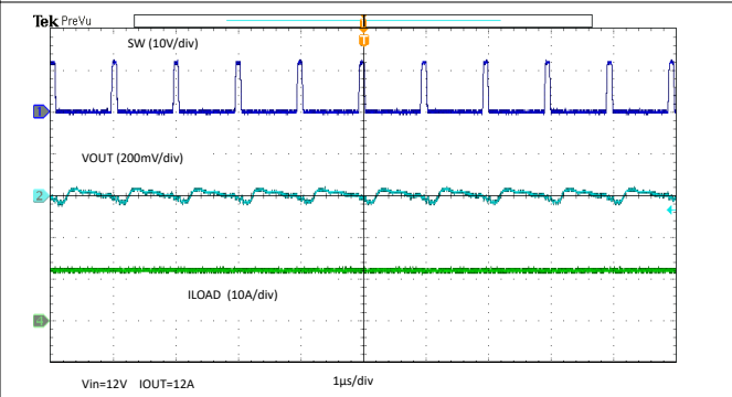
7-17. Output Ripple – Full Load
