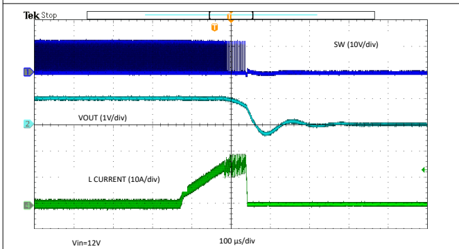
7-20. Overcurrent Protection – Overload
