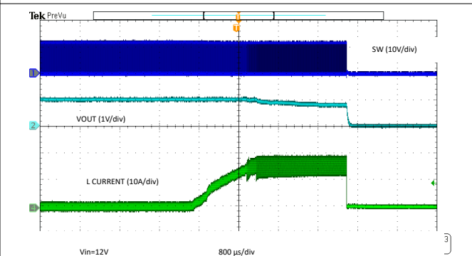
7-21. Overcurrent Protection – Short
