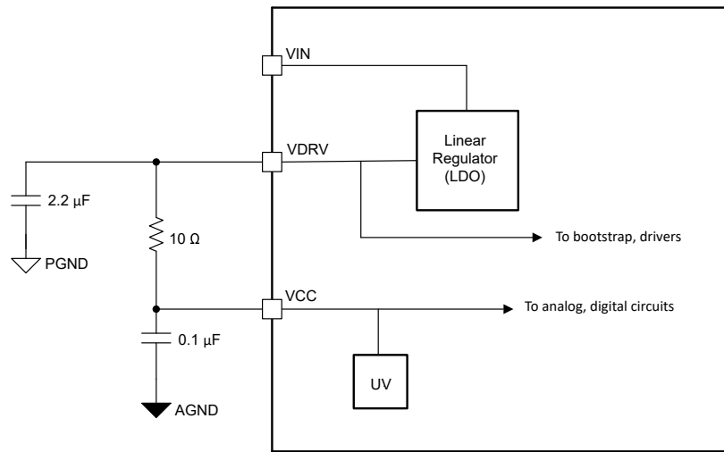
図 6-1. Device Bypassing
