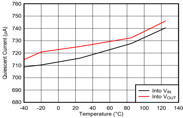
6-13. Quiescent Current vs Temperature
