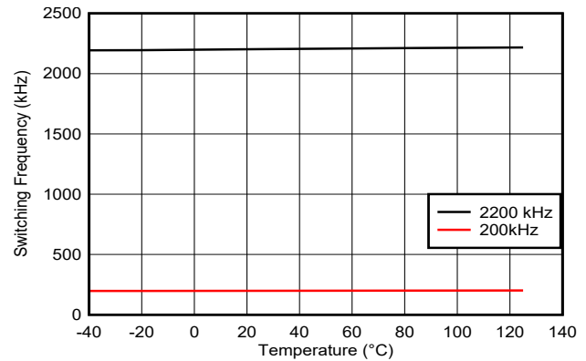
6-16. Switching Frequency vs Temperature
