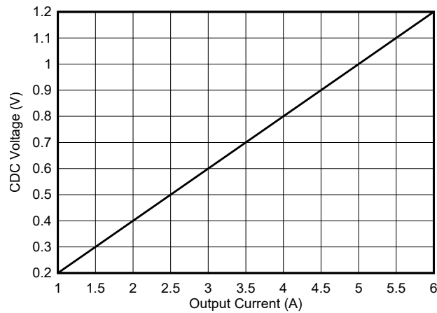
6-17. CDC Voltage vs Output Current with R_{SENSE} = 10\text{ m}\Omega
