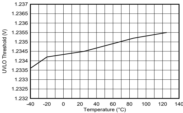
6-15. ENABLE/UVLO Rising Threshold vs Temperature
