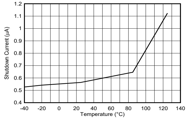
6-14. Shutdown Current vs Temperature
