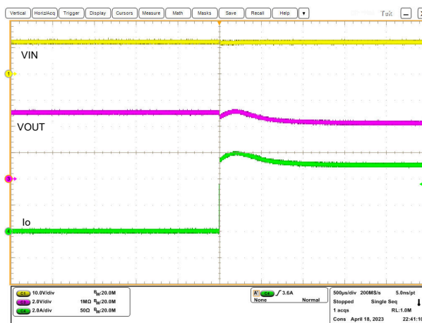
8-12. Output Current Limit Waveforms in V_{IN} = 12\text{ V} , V_{OUT} = 5\text{ V} , R_{LOAD} = 0.8\ \Omega , R_{SNS} = 10\text{ m}\Omega , FPWM
