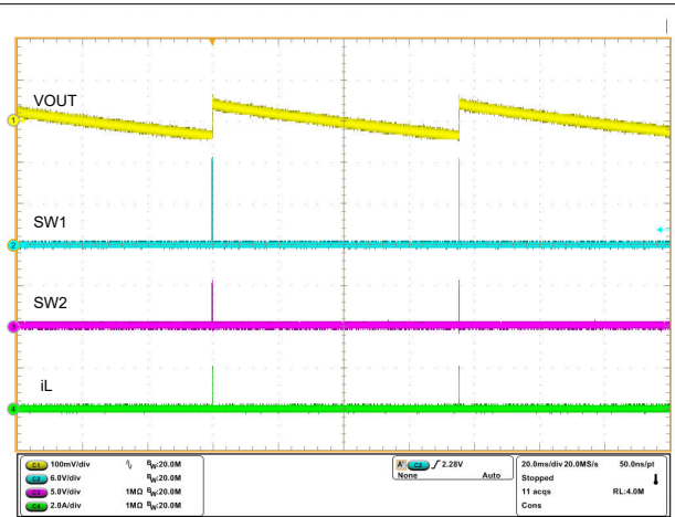
8-3. Switching Waveforms in V_{IN} = 12\text{ V} , V_{OUT} = 5\text{ V} , I_O = 0\text{ A} , PFM
