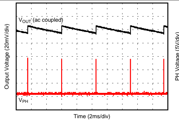
18. Output Ripple, I_{OUT} = 0 \text{ mA}
