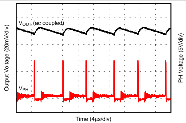
17. Output Ripple, I_{OUT} = 30 \text{ mA}
