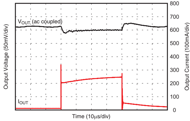
14. Transient Response, 2% to 50% Load Step
