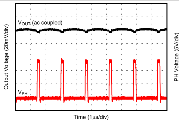
16. Output Ripple, I_{OUT} = 500 \text{ mA}
