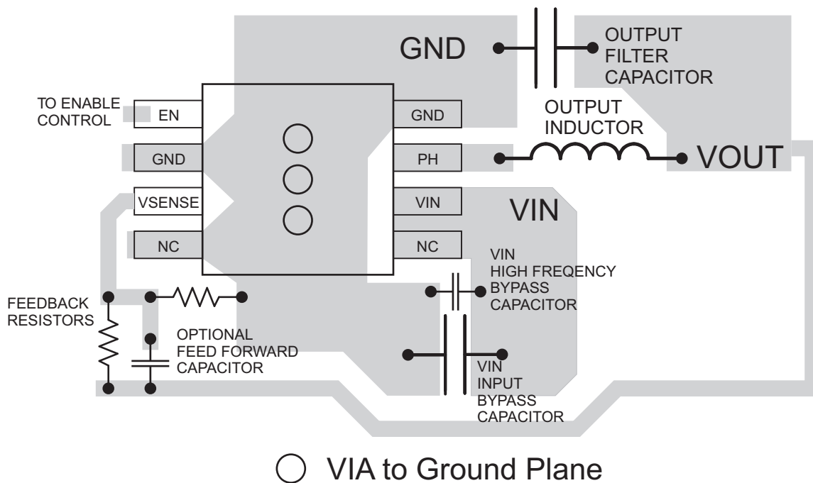
☒ 19. Layout Schematic
