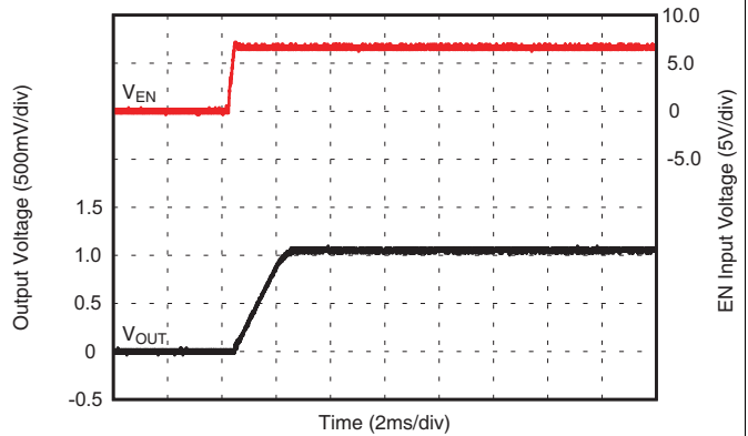
15. Start-Up Relative to EN
