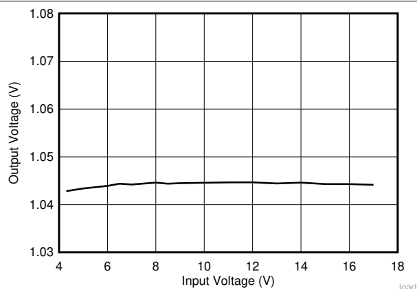
FIG 9-3. Load Regulation with Different Input Voltage
