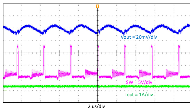
FIG 9-6. Output Voltage Ripple, I_{out} = 0.2\text{ A}
