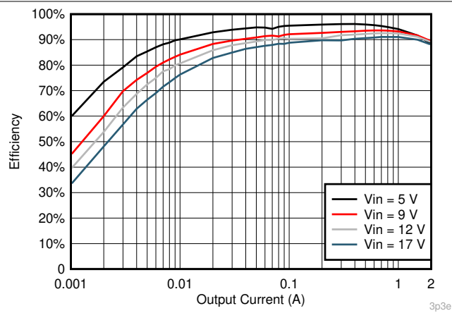
7-13. V_{OUT} = 3.3V Efficiency, L = 3.3\mu H
