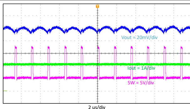
FIG 9-7. Output Voltage Ripple, I_{out} = 2\text{ A}
