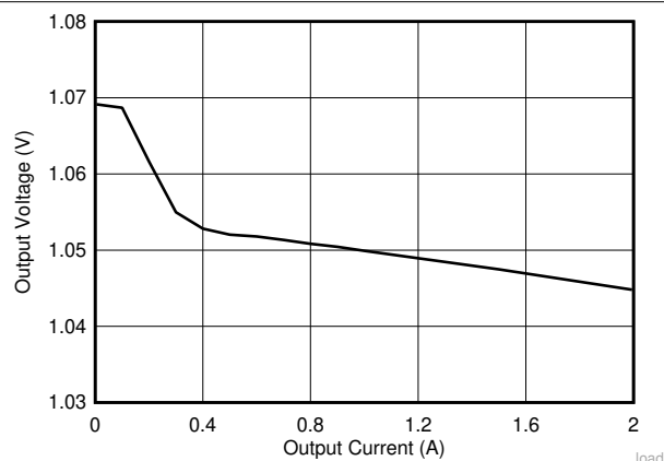
FIG 9-2. Load Regulation with Different Loading
