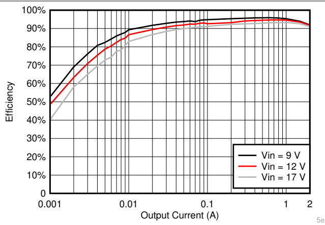
7-14. V_{OUT} = 5V Efficiency, L = 4.7\mu H
