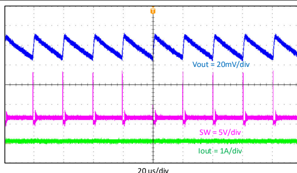
FIG 9-5. Output Voltage Ripple, I_{out} = 0.01\text{ A}
