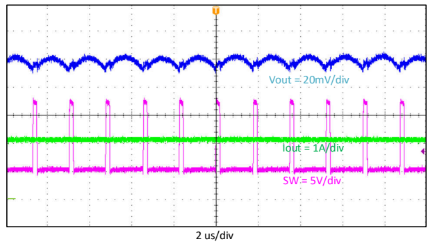
9-7. Output Voltage Ripple, I_{out} = 2\text{ A}
