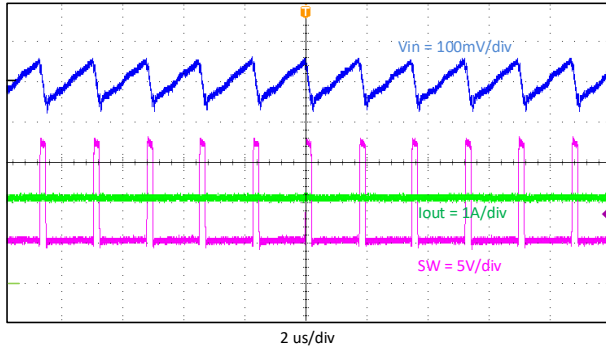
9-4. Input Voltage Ripple I_{out} = 2\text{ A}
