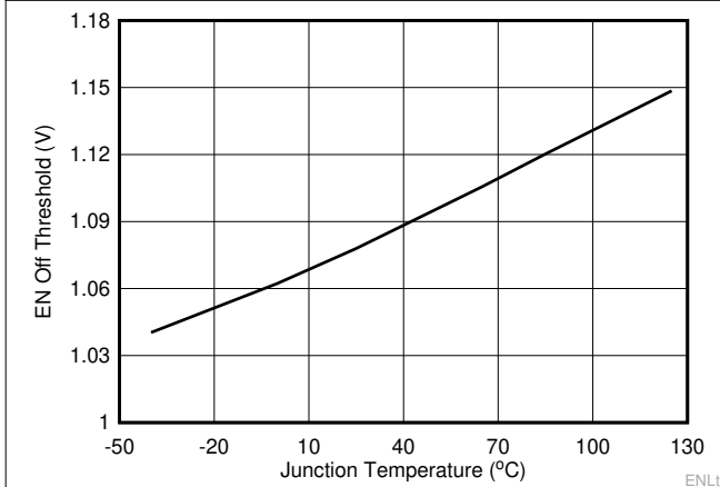
7-3. EN Off Threshold Voltage vs Junction Temperature
