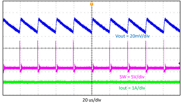
9-5. Output Voltage Ripple, I_{out} = 0.01\text{ A}
