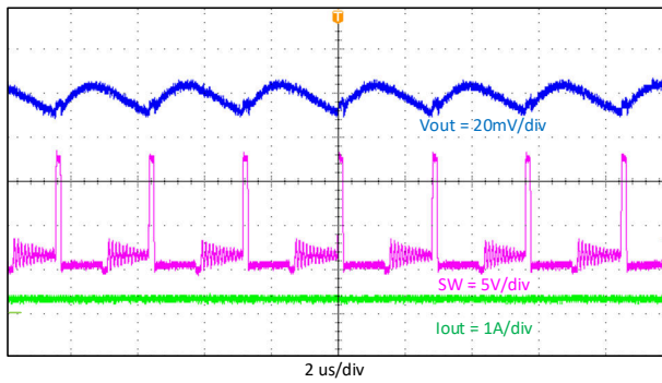
9-6. Output Voltage Ripple, I_{out} = 0.2\text{ A}
