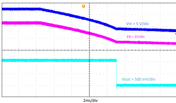
8-12. Shutdown Relative to V_{IN}
